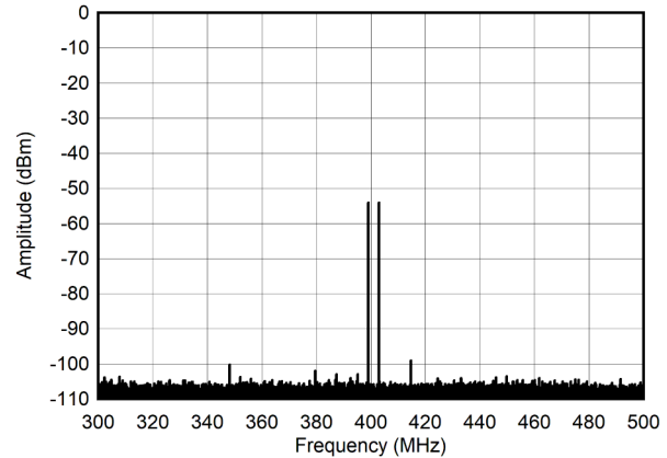
Figure 5-265. Dual Tone Spectrum at 400 MHz and -60 dBFS (±100MHz)
