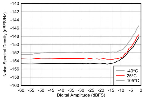
Figure 5-553. NSD vs Digital Amplitude and Temperature at 7.1 GHz
