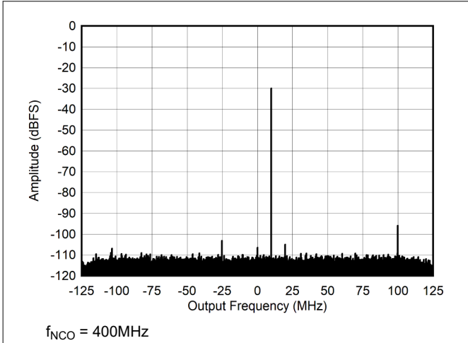
Figure 4-41. RX Output FFT at 405 MHz and -30dBFS
