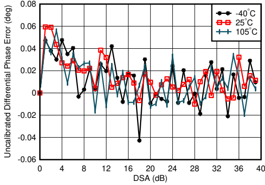
3.5 GHz Matching, 1TX Differential Phase Error = \text{Phase}_{OUT}(\text{DSA Setting} - 1) - \text{Phase}_{OUT}(\text{DSA Setting})
