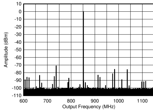
Figure 4-350. TX Single Tone (-6 dBFS) Output Spectrum at 0.85 GHz ( \pm 300 MHz)
