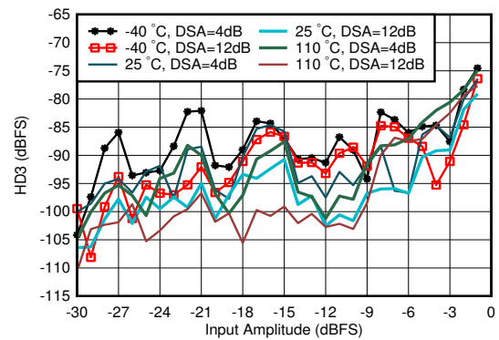
With 1.8 GHz matching, f_{\text{in}} = 1900\text{ MHz} , DDC bypass mode (TI only mode for characterization)
