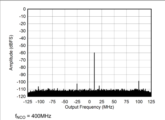
Figure 4-42. RX Output FFT at 405 MHz and -60dBFS
