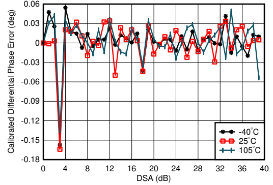
3.5 GHz Matching, 1TX, Calibrated at 25°C Differential Phase Error = \text{Phase}_{OUT}(\text{DSA Setting} - 1) - \text{Phase}_{OUT}(\text{DSA Setting})
