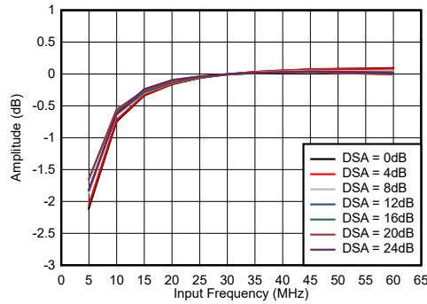
Figure 4-1. RX In-Band Gain Flatness, f_{\text{IN}} = 30 MHz
