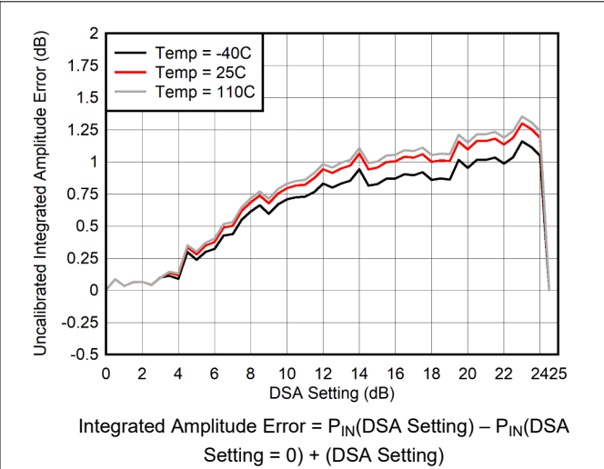
Figure 4-32. RX Uncalibrated Integrated Amplitude Error vs DSA Setting at 400 MHz
