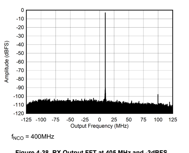
Figure 4-38. RX Output FFT at 405 MHz and -3dBFS
