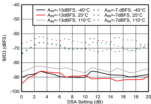
Figure 5-452. RX IMD3 vs DSA Setting at 9.6 GHz
