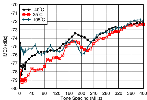
Figure 5-23. TX IMD3 vs Tone Spacing and Channel at 0.85 GHz
