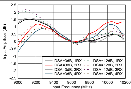
Figure 5-444. RX Input Amplitude vs Frequency
