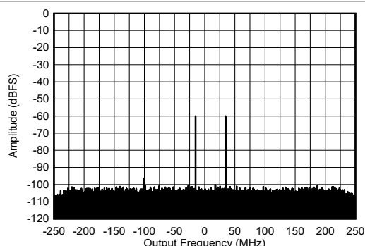
Figure 5-443. RX Dual Tone Output FFT at 8.11 GHz
