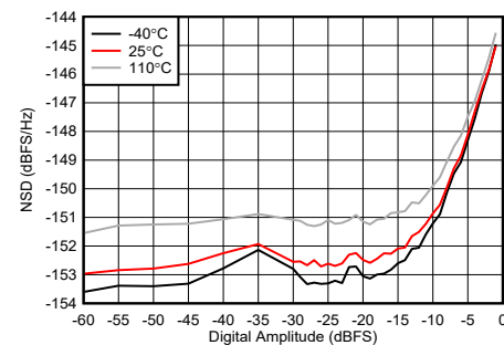
Figure 4-260. TX NSD vs Digital Amplitude at 9.61 GHz
