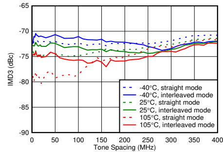
Figure 4-101. TX IMD3 vs Tone Spacing and Temperature
