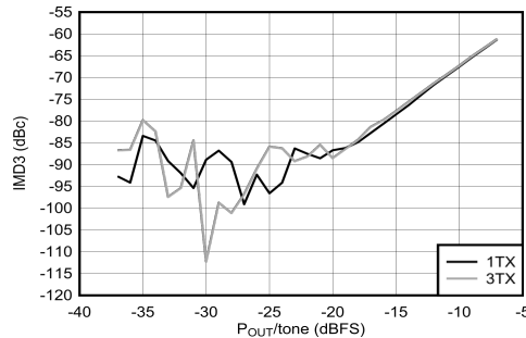
Figure 4-100. TX IMD3 vs Digital Level at 2.6 GHz
