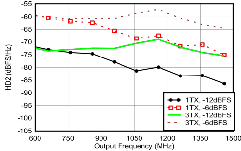
Matching at 0.8 GHz, f_{\text{DAC}} = 5898.24 GSPS, straight mode
