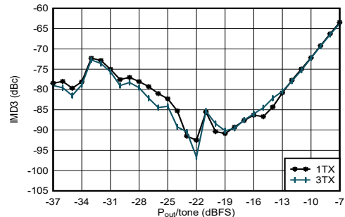
Figure 4-30. TX IMD3 vs Digital Level at 0.85 GHz
