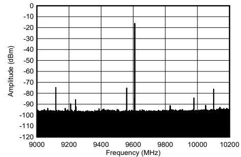
Figure 4-268. TX Single Tone Spectrum at 9.61 GHz and -6 dBFS (1.2 GHz BW)
