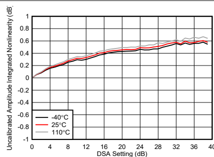
Figure 4-193. TX DSA Uncalibrated Amplitude Integrated Nonlinearity at 8.11 GHz
