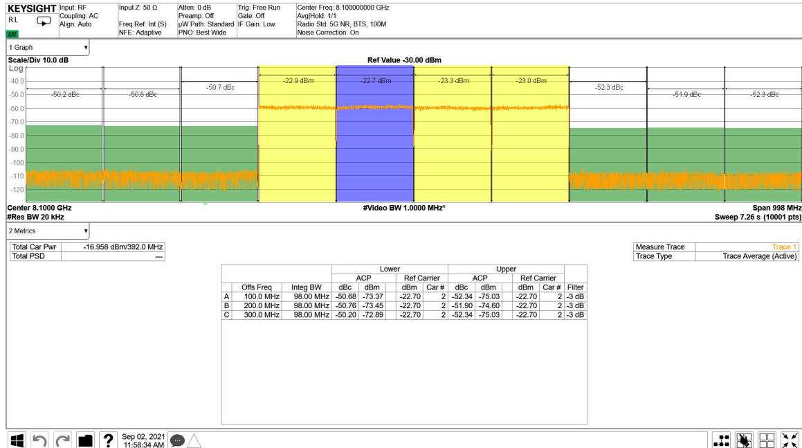
Figure 4-231. TX 4x100 MHz NR Output Spectrum 8.11 GHz
