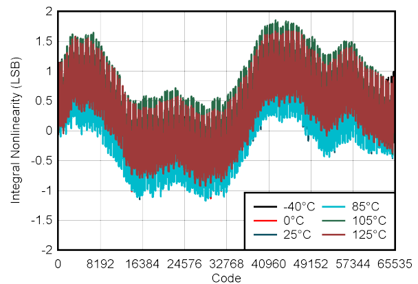
Figure 6-6. DAC INL vs Digital Input Code
