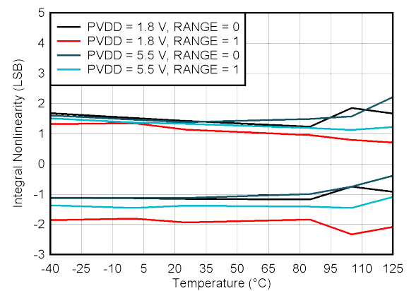
Figure 6-8. MIN and MAX DAC INL Range vs Temperature
