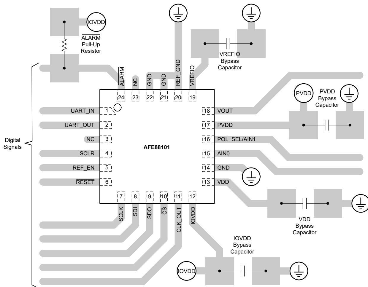
Figure 8-8. Layout Example
