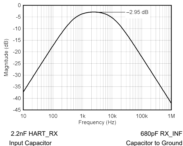
Figure 5-44. HART Internal Mode First Stage Band-Pass Filter Response (From HART_RX Signal to RX_INF Pin)
