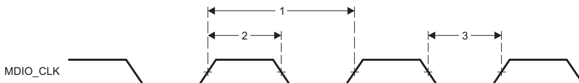
Figure 7-103. PRU-ICSS MDIO_CLK Timing
