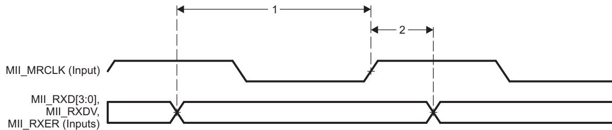
Figure 7-107. PRU-ICSS MII_RXD[3:0], MII_RXDV, and MII_RXER Timing
