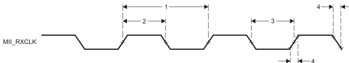
Figure 7-105. PRU-ICSS MII_RXCLK Timing
