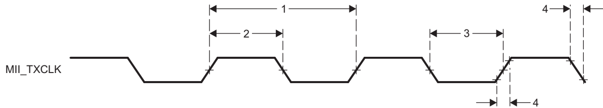
Figure 7-106. PRU-ICSS MII_TXCLK Timing
