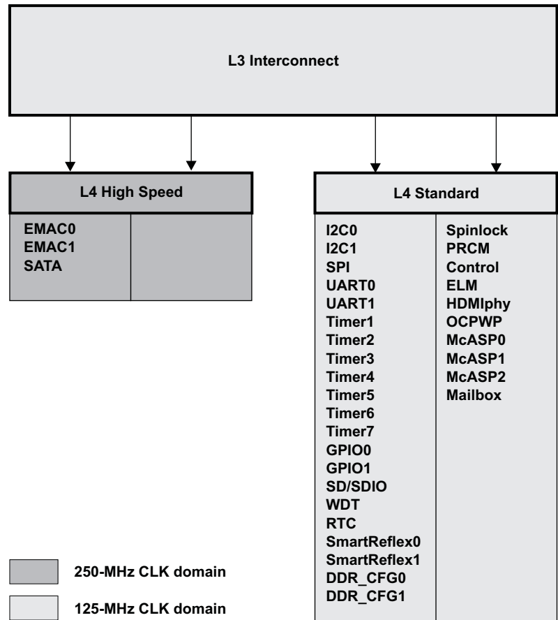
Figure 7-2. L4 Architecture
