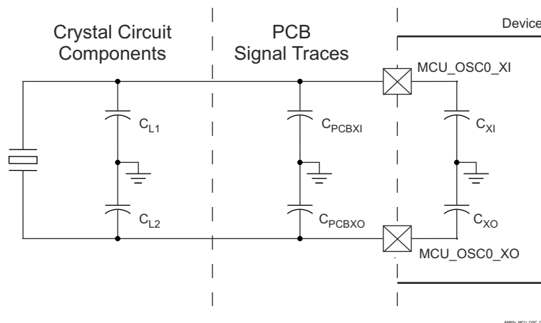
Figure 6-18. Load Capacitance
