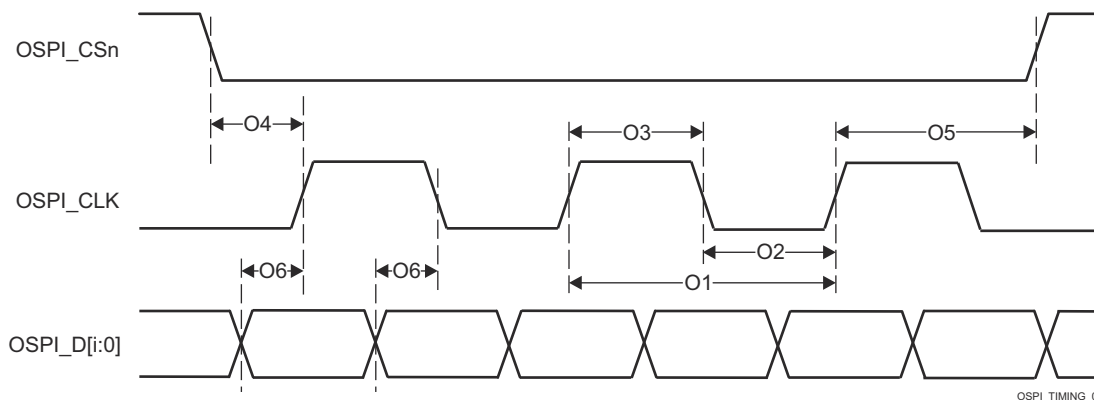
Figure 6-105. OSPI0 Switching Characteristics – PHY DDR
