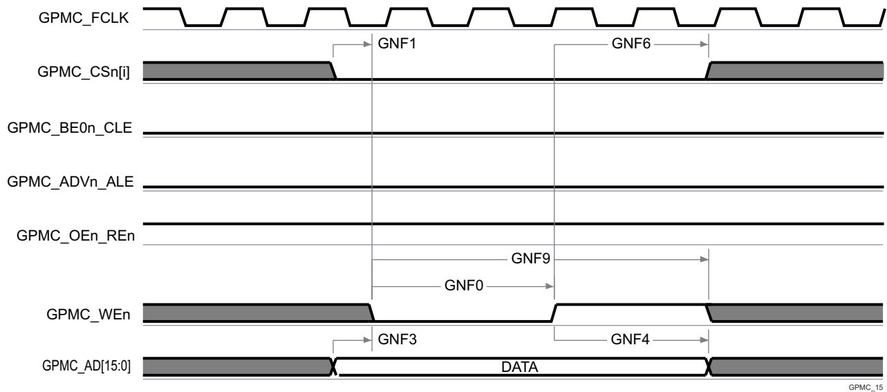
Figure 6-59. GPMC and NAND Flash — Data Read Cycle
