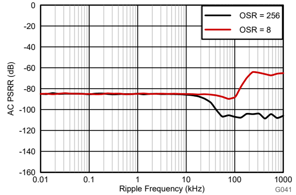
Figure 5-16. Power-Supply Rejection Ratio vs Ripple Frequency
