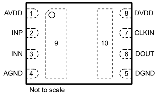
Figure 4-1. DEN Package, 8-Pin VSON (Top View)
