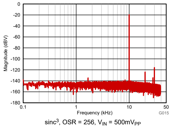
Figure 5-35. Frequency Spectrum With 10kHz Input Signal
