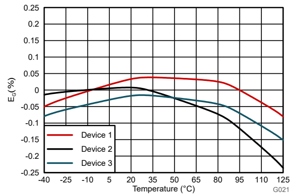
Figure 6-19. Gain Error vs Temperature
