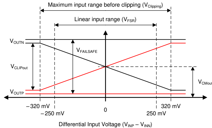
Figure 7-2. Output Behavior of the AMC1301-Q1
