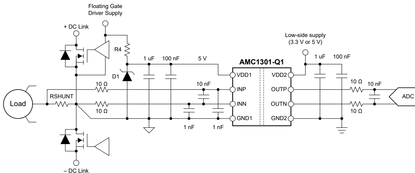
Figure 8-1. Using the AMC1301-Q1 for Current Sensing in a Typical Application
