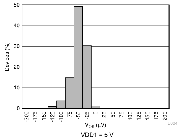
Figure 6-8. Input Offset Voltage Histogram
