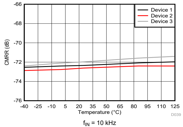
Figure 6-30. Common-Mode Rejection Ratio vs Temperature
