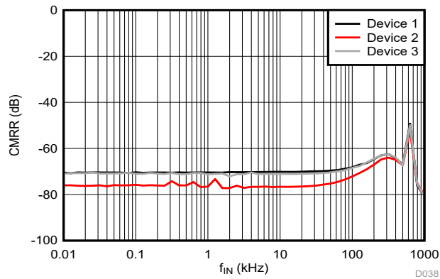
Figure 6-29. Common-Mode Rejection Ratio vs Input Frequency
