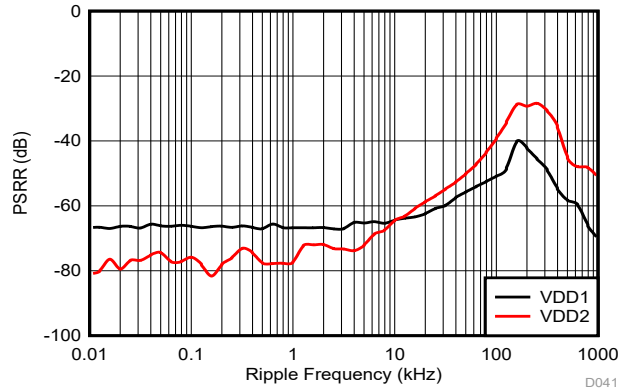
Figure 6-31. Power-Supply Rejection Ratio vs Ripple Frequency
