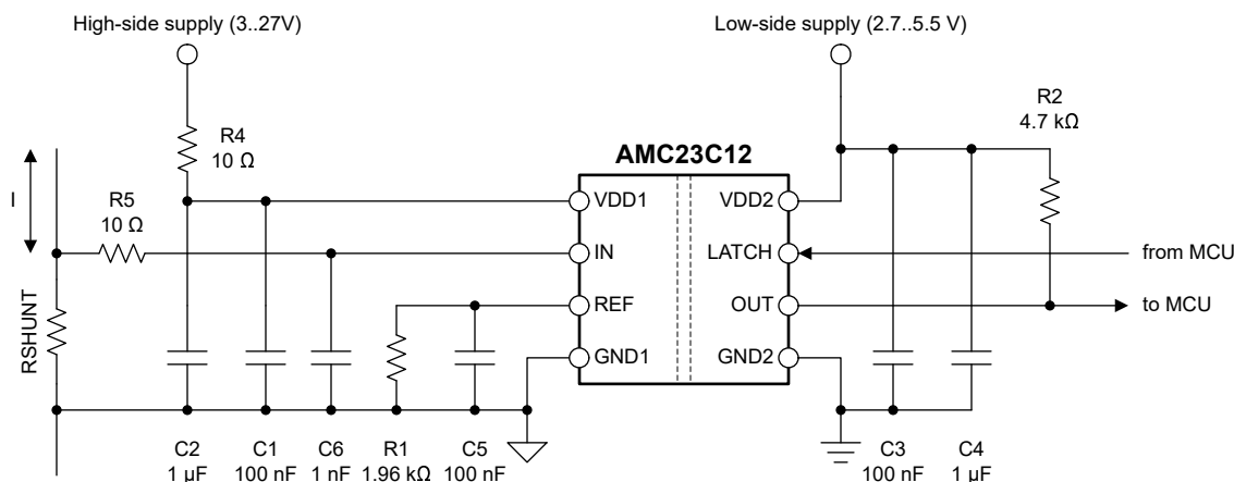
Figure 7-6. Decoupling of the AMC23C12
