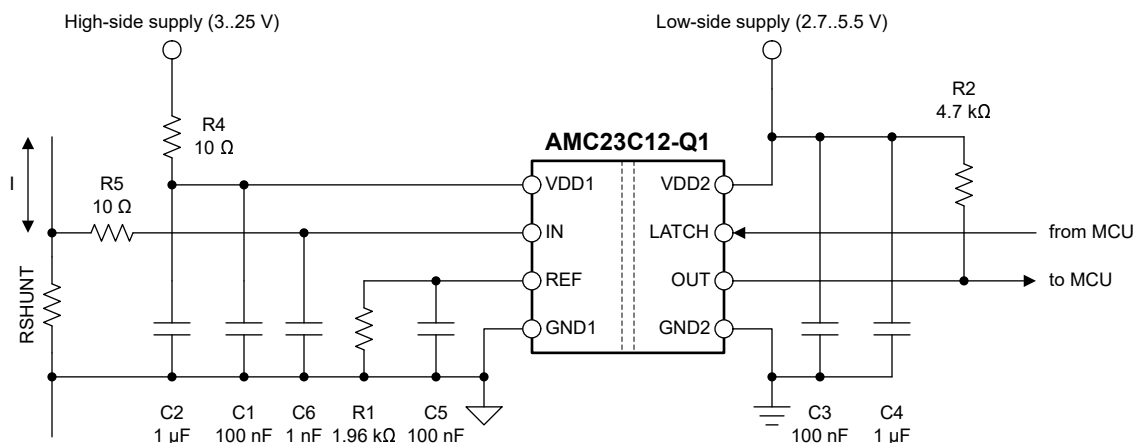
Figure 7-6. Decoupling of the AMC23C12-Q1
