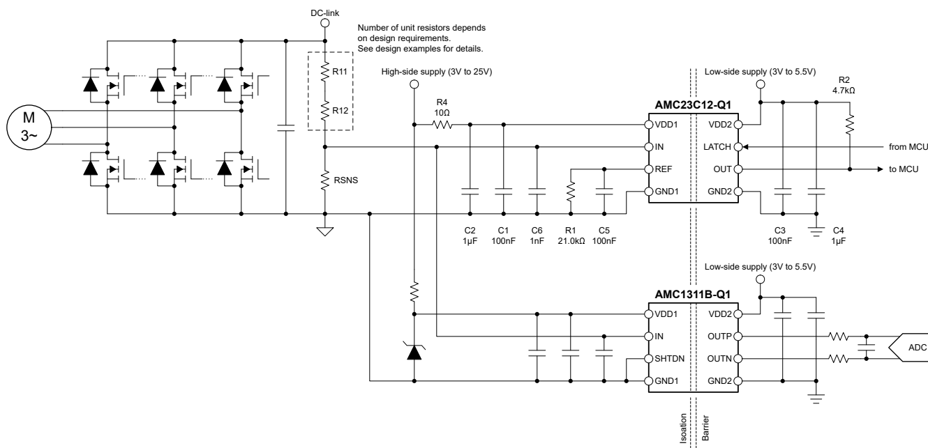
Figure 7-2. Using the AMC23C12-Q1 for Overvoltage Detection
