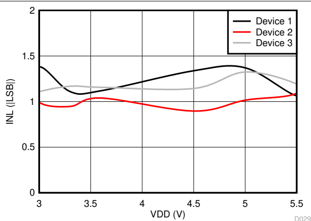
Figure 6-17. Integral Nonlinearity vs Supply Voltage
