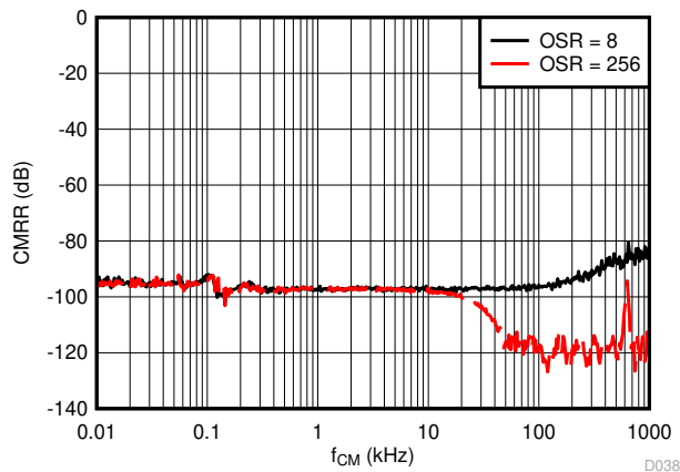
Figure 6-36. Common-Mode Rejection Ratio vs Input Signal Frequency
