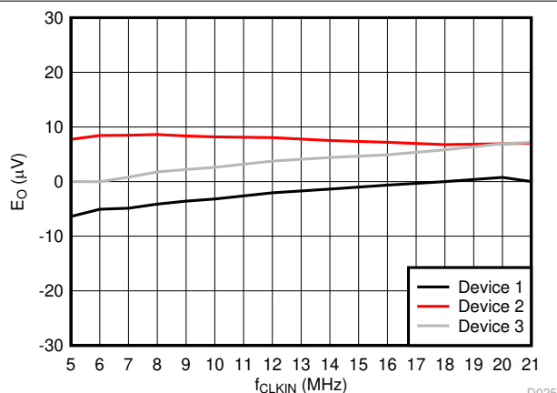
Figure 6-9. Offset Error vs Input Clock Frequency
