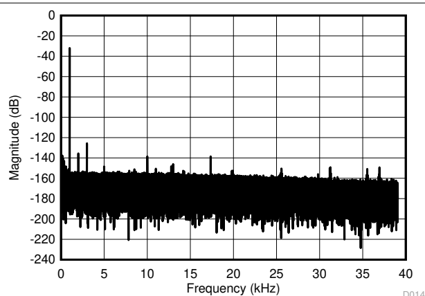
Figure 6-34. Output Frequency Spectrum With a 1-kHz Input Signal
