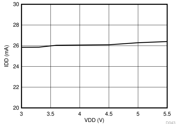
Figure 6-38. Supply Current vs Supply Voltage
