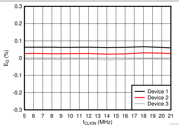
Figure 6-12. Gain Error vs Input Clock Frequency
