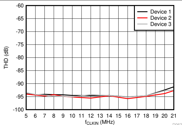
Figure 6-26. Total Harmonic Distortion vs Input Clock Frequency
