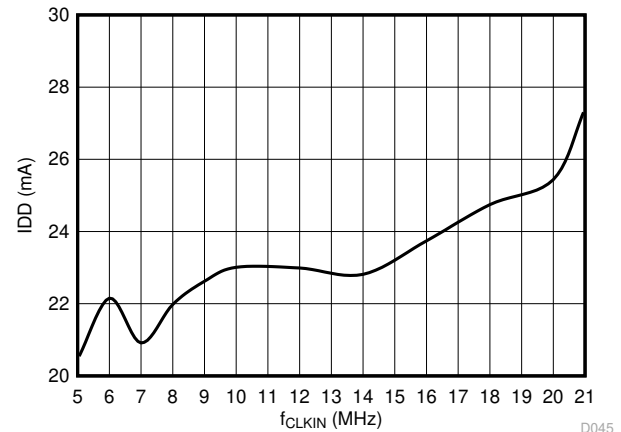
Figure 6-39. Supply Current vs Input Clock Frequency
