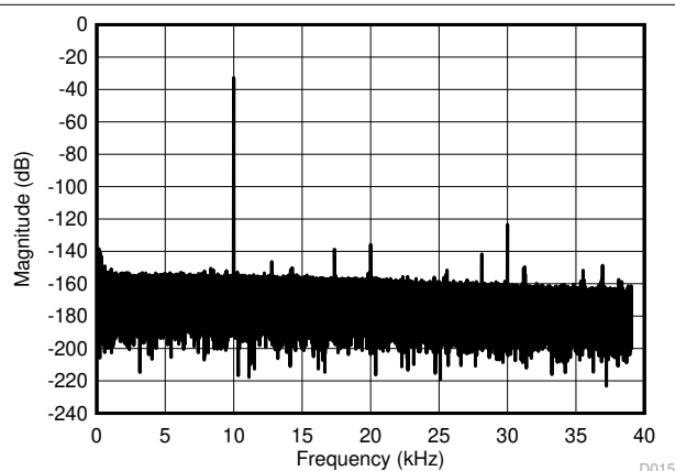
Figure 6-35. Output Frequency Spectrum With a 10-kHz Input Signal
