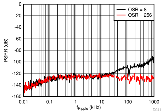
Figure 6-37. Power-Supply Rejection Ratio vs Ripple Frequency
