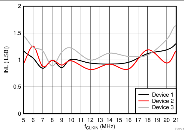
Figure 6-16. Integral Nonlinearity vs Input Clock Frequency
