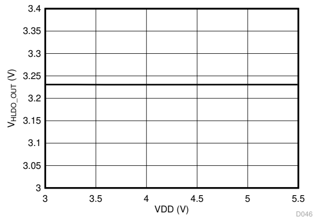
Figure 6-41. High-Side LDO Output Voltage vs Supply Voltage
