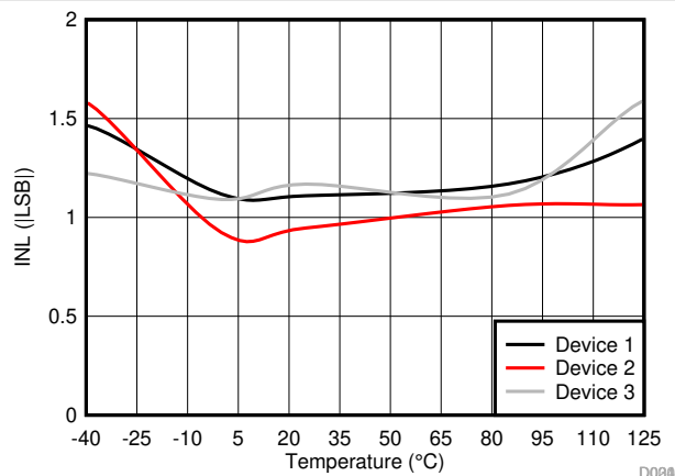
Figure 6-18. Integral Nonlinearity vs Temperature
