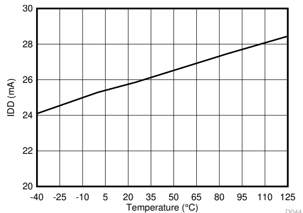
Figure 6-40. Supply Current vs Temperature
