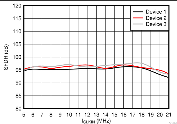
Figure 6-31. Spurious-Free Dynamic Range vs Input Clock Frequency
