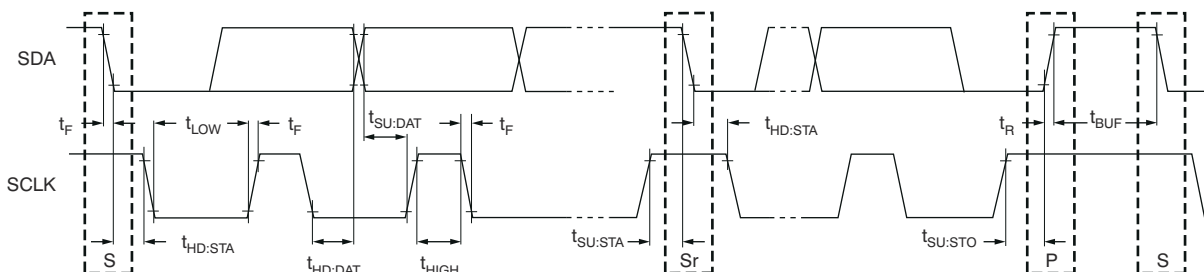
Figure 7-1. Timing Specification
