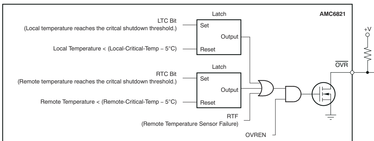
Figure 8-20. \overline{\text{OVR}} Pin
