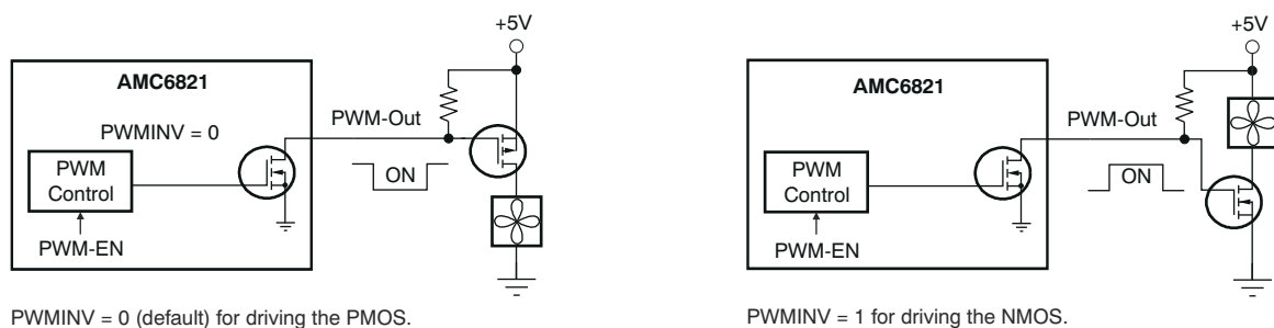
Figure 8-5. PWM Output
