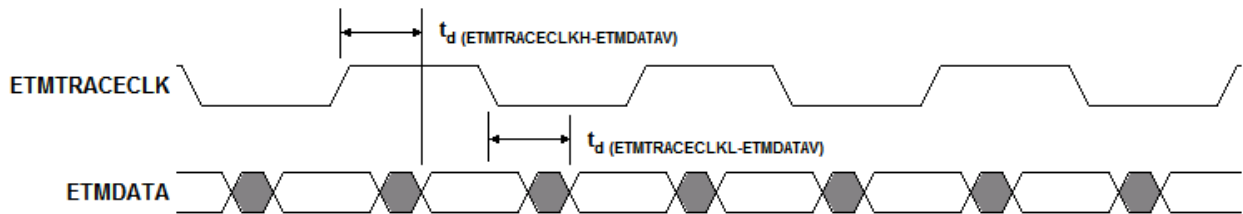
Figure 6-21. ETMDATA Timing
