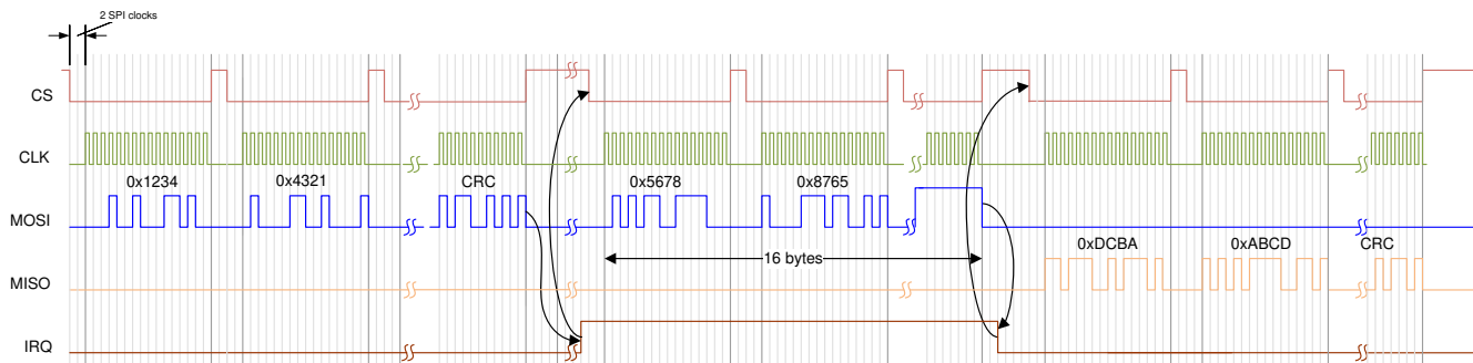
Figure 6-14. SPI Communication
