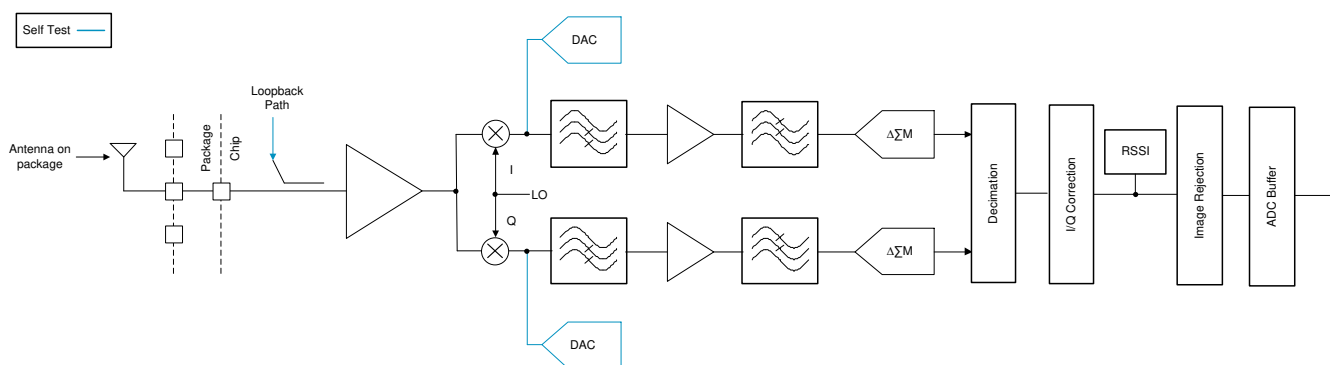
Figure 7-3. Receive Subsystem (Per Channel)
