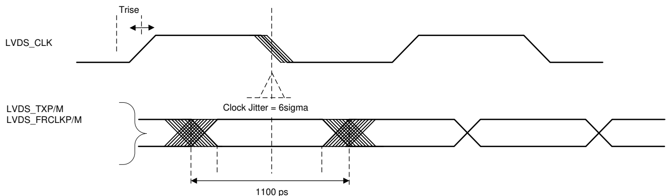
Figure 7-22. Timing Parameters
