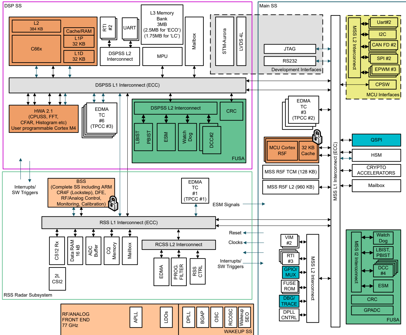
Figure 8-5. Processor Subsystem
