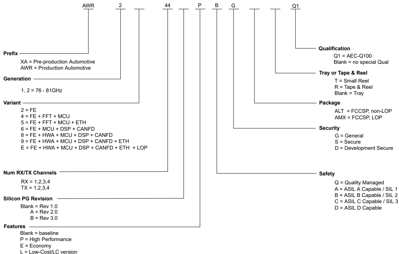
Figure 11-1. Device Nomenclature
