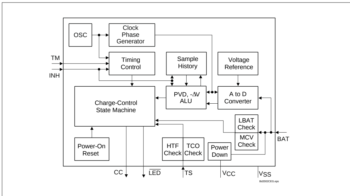
Figure 3. Block Diagram
