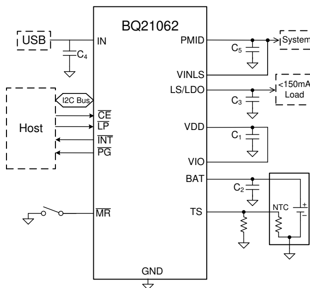
Simplified Schematic
