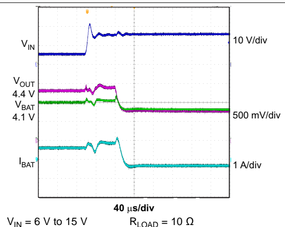
Figure 32. OVP Fault
