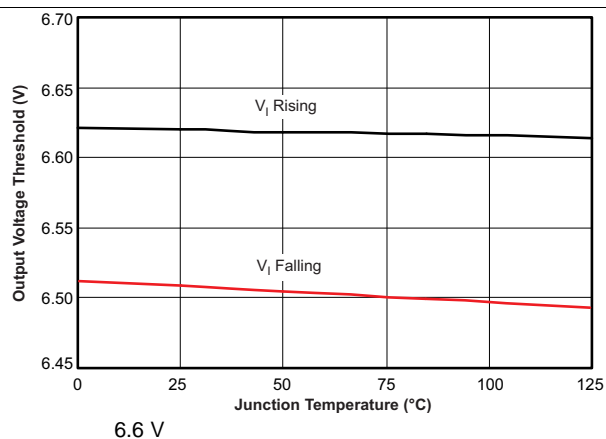
Figure 10. Overvoltage Protection Threshold vs Temperature
