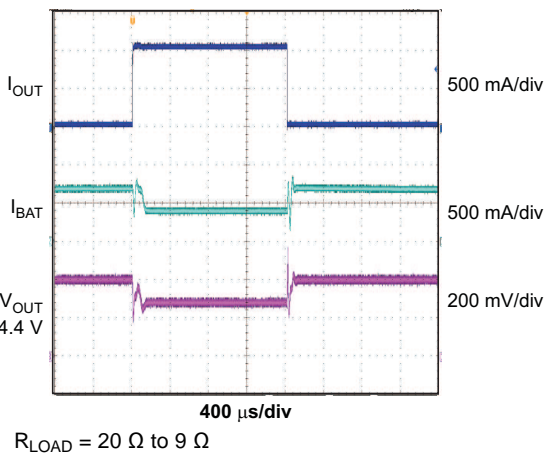
Figure 30. Entering And Exiting DPPM Mode
