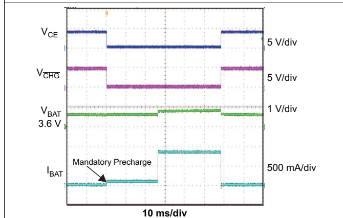
Figure 29. Battery Detection Battery Removed
