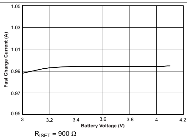
Figure 11. Fastcharge Current vs Battery Voltage
