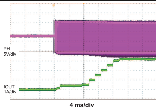
Figure 1. Power Up (ISET = 0)
