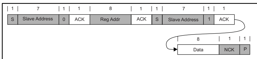
Figure 19. Single Read
