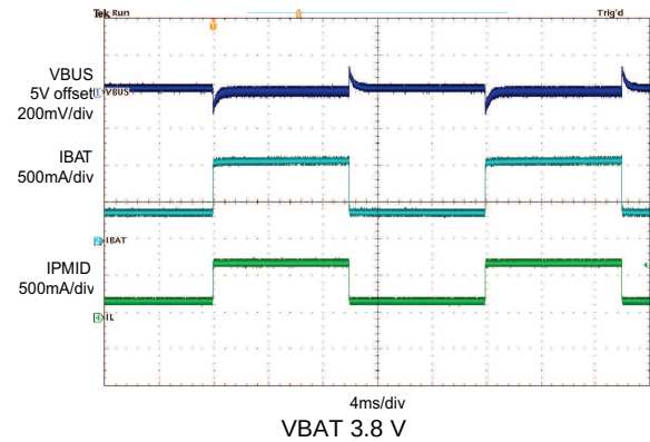
Figure 41. Boost Mode Load Transient
