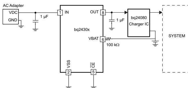
APPLICATION SCHEMATIC
