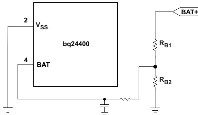
Figure 5. Battery Voltage Divider and Filter
