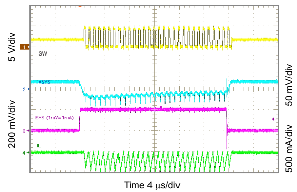
Figure 10-35. 3.3 V_{SYS} Load Transient, 0 to 50 mA
