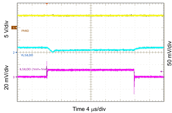
Figure 10-49. 3.3 V LSDO Load Transient, 0 to 10 mA
