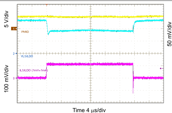
Figure 10-54. 3.3 V LSDO Load Transient, 0 to 100 mA
