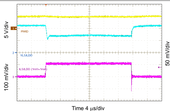
Figure 10-53. 2.5 V LSDO Load Transient, 0 to 100 mA
