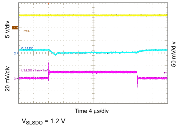
Figure 10-46. 1.2 V LSLDO Load Transient, 0 to 10 mA
