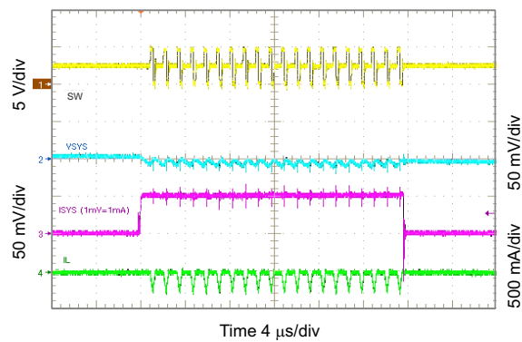
Figure 10-32. 1.8 V_{SYS} Load Transient, 0 to 50 mA
