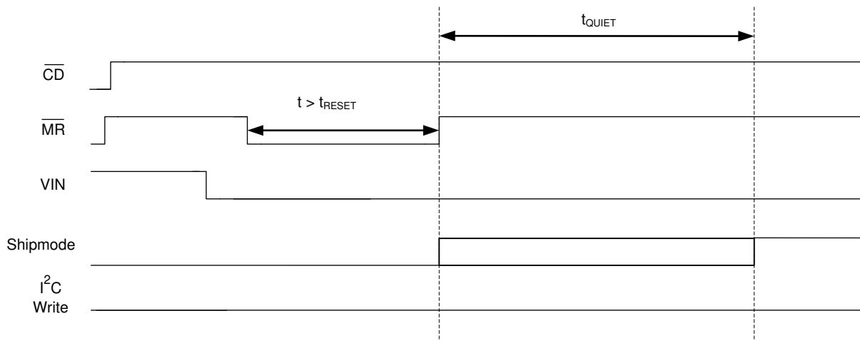
Figure 9-2. \overline{CD} , \overline{MR} and V_{IN} Sequencing for Ship Mode Entry Through Long MR button press
