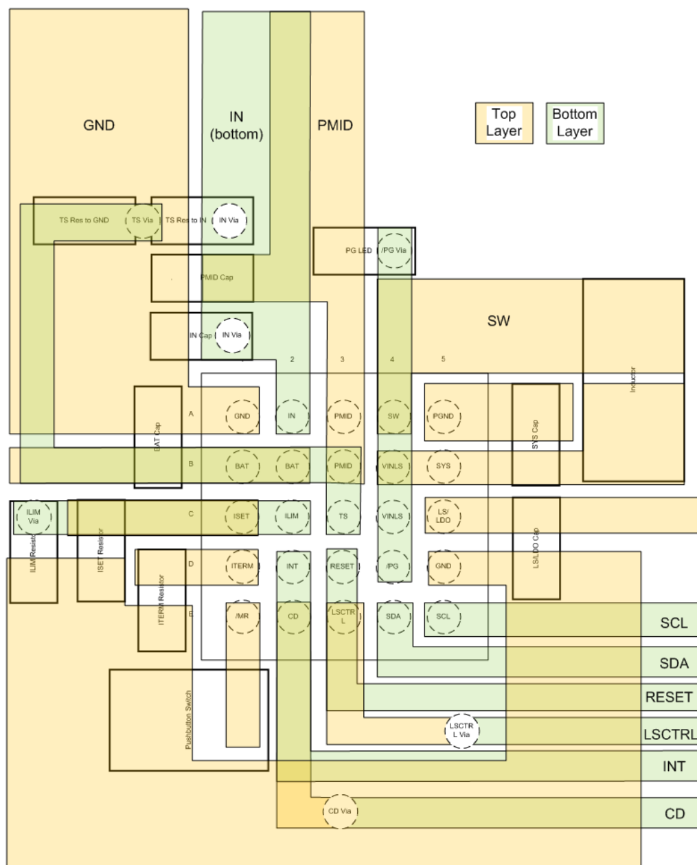
Figure 12-1. BQ25125 Layout
