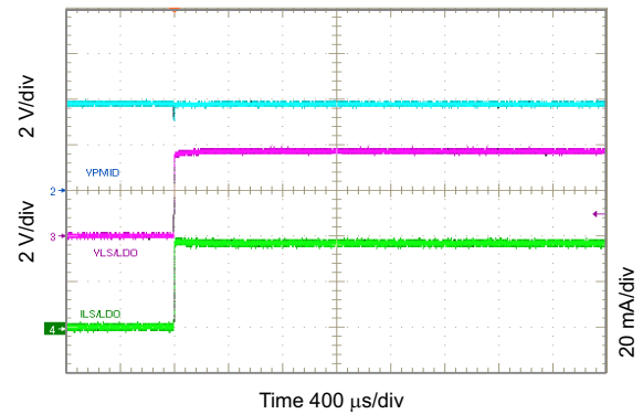
Figure 10-44. Startup Showing SS on LS/LDO Output
