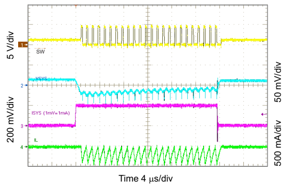
Figure 10-34. 2.5 V_{SYS} Load Transient, 0 to 50 mA
