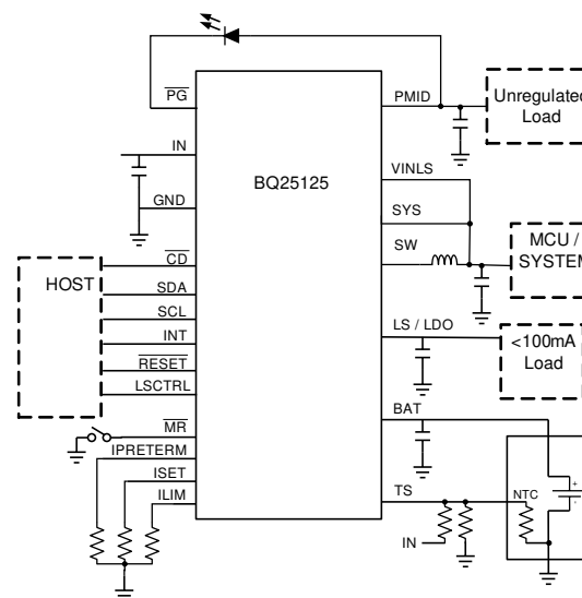
Simplified Schematic
