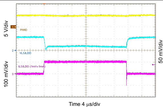
Figure 10-51. 1.2 V LSDO Load Transient, 0 to 100 mA
