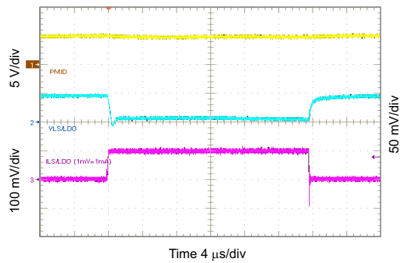
Figure 10-50. 0.8 V LSDO Load Transient, 0 to 100 mA
