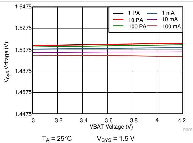
Figure 10-19. 1.5 V sys Line Regulation
