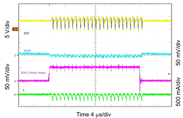
Figure 10-33. 2.1 V_{SYS} Load Transient, 0 to 50 mA
