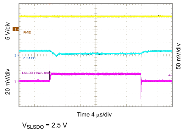
Figure 10-48. 2.5 V LSLDO Load Transient, 0 to 10 mA
