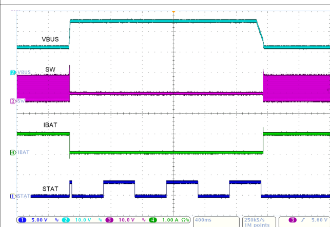
Figure 10-3. Charge Cycle
