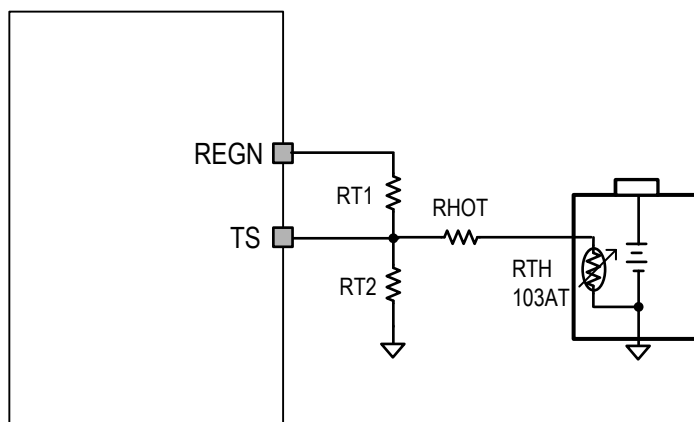
Figure 9-2. Battery Temperature Sensing Circuit
