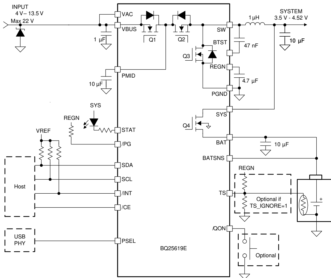
Figure 9-2. BQ25619E Application Diagram
