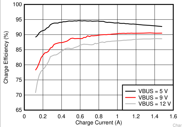
Figure 7-2. Charge Efficiency
