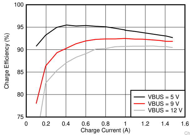
Figure 7-1. Charge Efficiency
