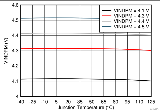
Figure 7-6. VINDPM vs Junction Temperature
