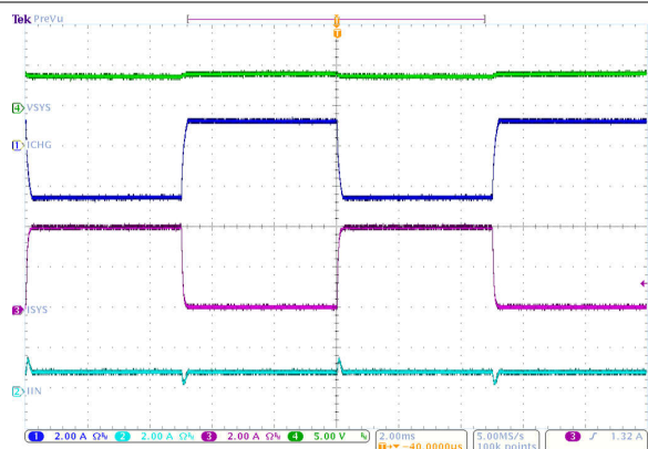
Figure 9-7. System Load Transient Response
