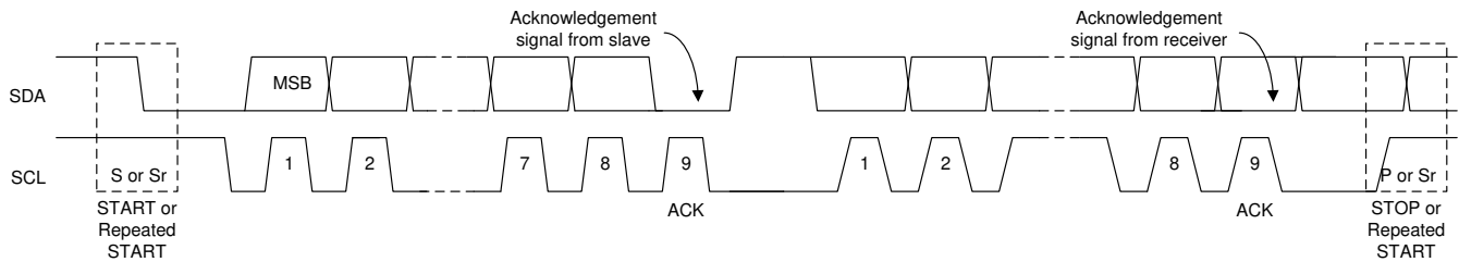
Figure 8-8. Data Transfer on the I²C Bus
