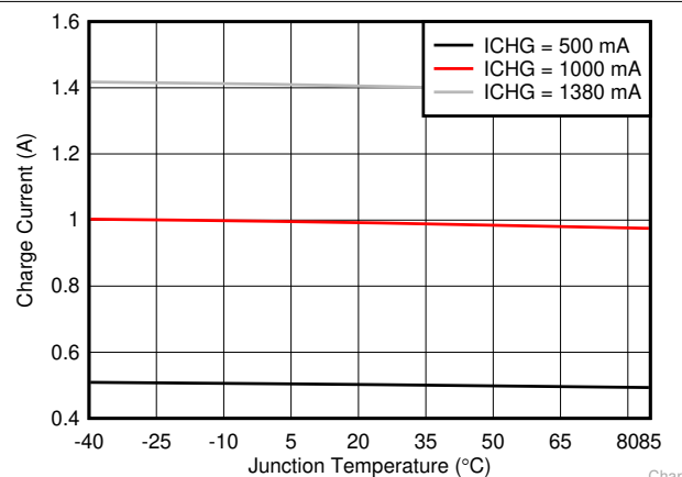
Figure 7-5. Charge Current vs Junction Temperature
