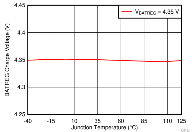
Figure 7-4. Battery Charge Voltage vs Junction Temperature
