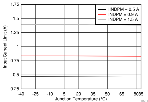
Figure 7-8. Input Current Limit vs Junction Temperature
