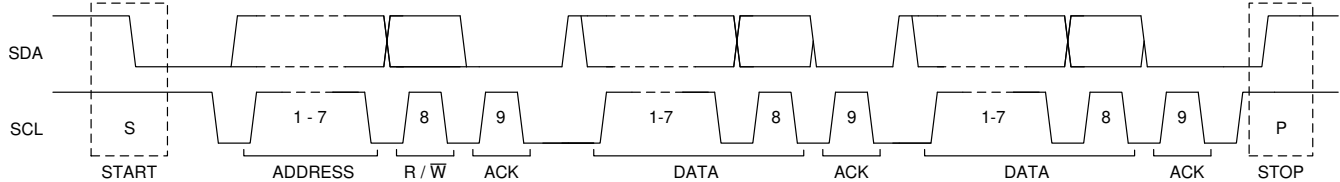
Figure 8-9. Complete Data Transfer
