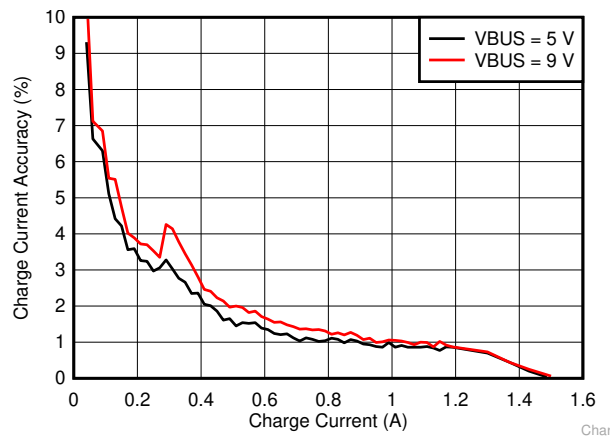
Figure 7-3. Charge Current Accuracy
