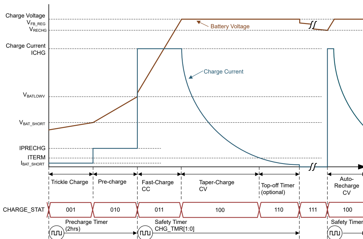
Figure 8-3. Typical Li-Ion Battery Charging Profile
