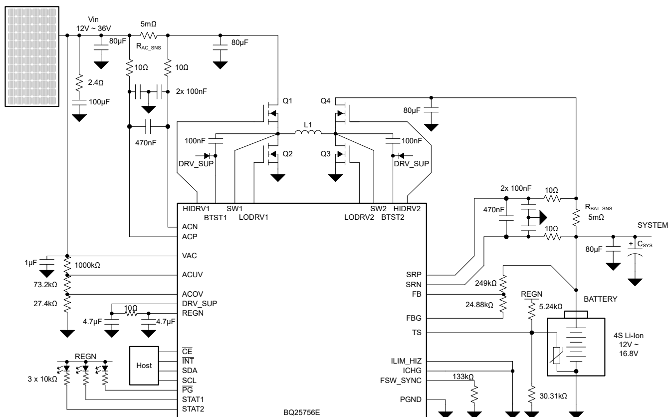
Figure 9-1. BQ25756E: Solar Charging with Autonomous MPPT Algorithm to Charge 4s Battery with Maximum 15-A Charge Current
