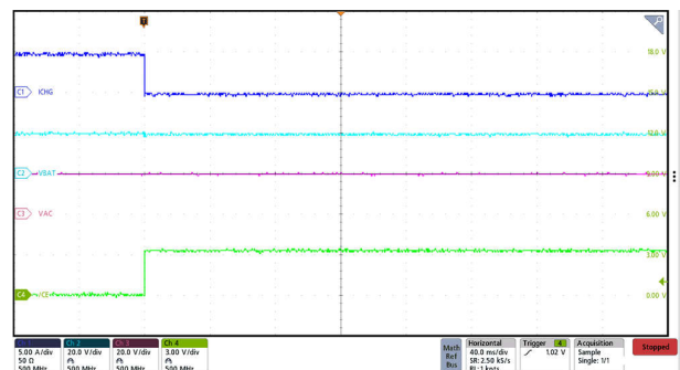
Figure 9-8. Charge Disable via \overline{CE} Pin with 5-A ICHG
