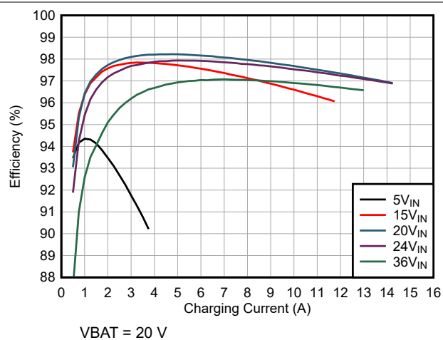
Figure 7-2. Charge Efficiency vs Charge Current (5s battery configuration)
