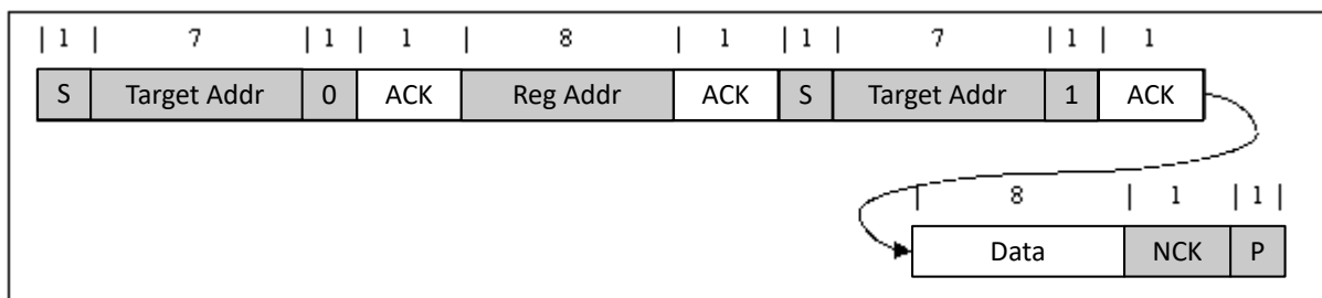
Figure 8-12. Single Read
