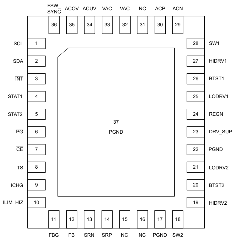
Figure 6-1. BQ25756E, RRV Package 36-pin VQFN Top View
