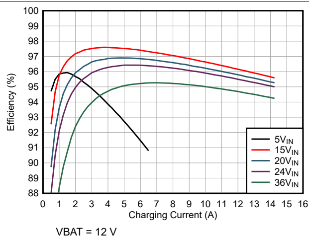
Figure 7-1. Charge Efficiency vs Charge Current (3s battery configuration)
