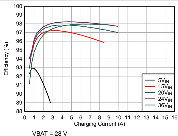
Figure 7-3. Charge Efficiency vs Charge Current (7s battery configuration)
