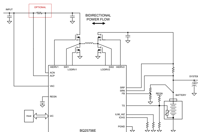
Simplified Schematic
