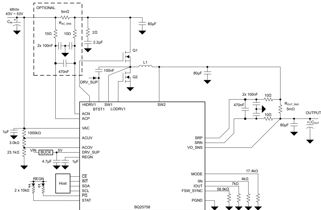
Figure 7-25. BQ25758: 48-Vin, Buck-Only with Configurable Output Voltage for USB-PD EPR, and 5-A Output Current
