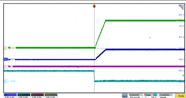
Figure 7-3. VAC Plug-In Power Up with 5-A Load
