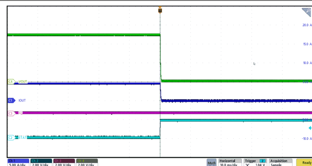
Figure 7-4. VAC Unplug Power Down with 5-A Load
