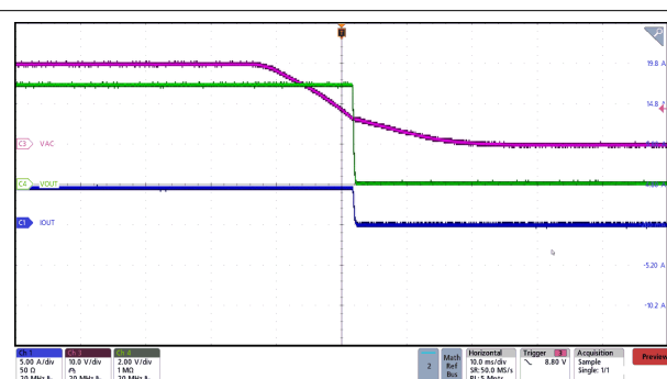
Figure 7-4. VAC Unplug Power Down with 5-A Load
