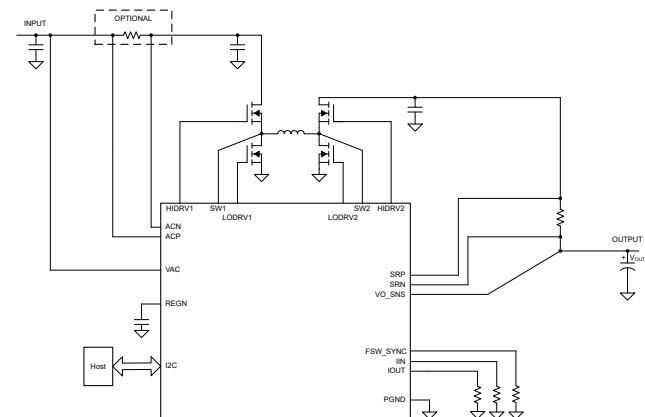
Simplified Schematic
