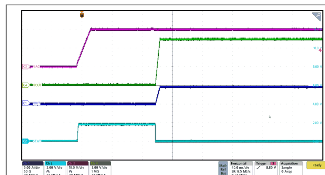
Figure 7-3. VAC Plug-In Power Up with 5-A Load
