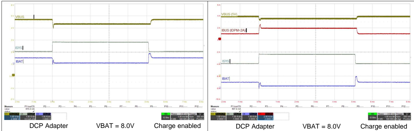
Figure 85. VINDPM Transient Response
