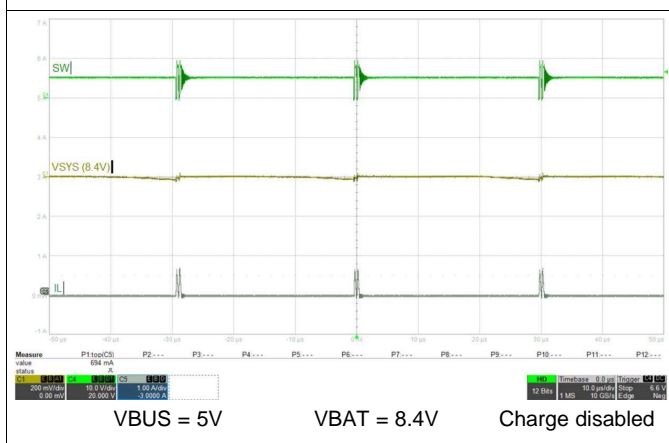
Figure 83. Boost Mode PFM Switching
