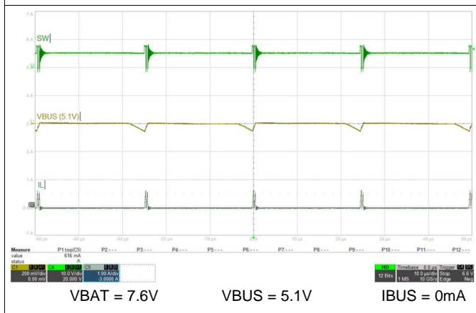
Figure 81. Buck Mode (OTG) PFM Switching
