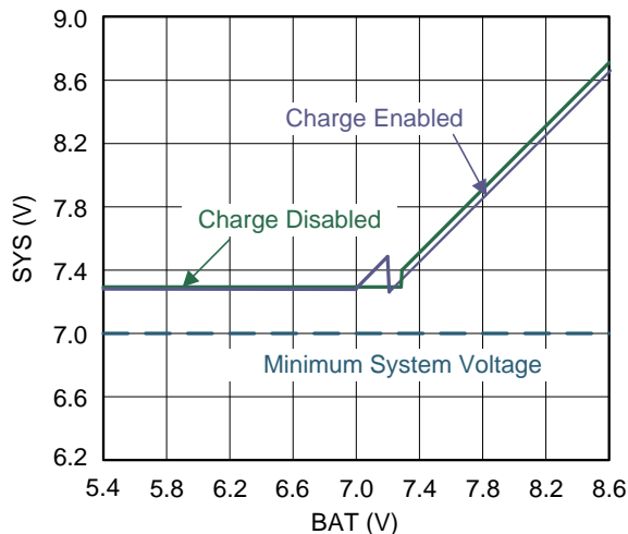
Figure 16. System Voltage vs. Battery Voltage
