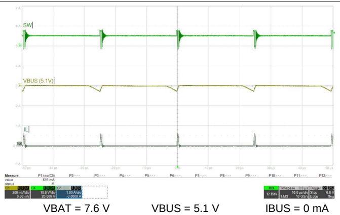
Figure 28. Buck Mode (OTG) PFM Switching
