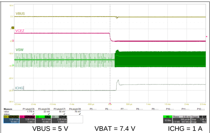
Figure 22. Charge Enable
