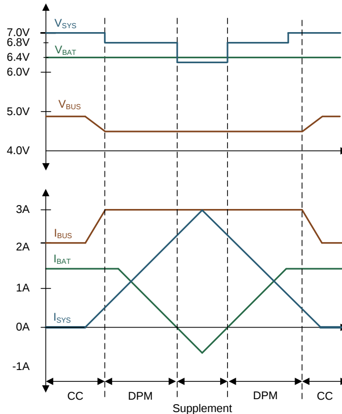
Figure 15. DPM Response
