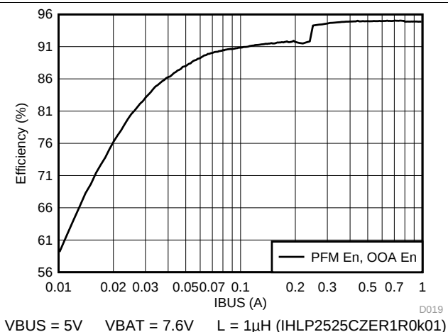
Figure 6. OTG Efficiency vs. VBUS Output Current
