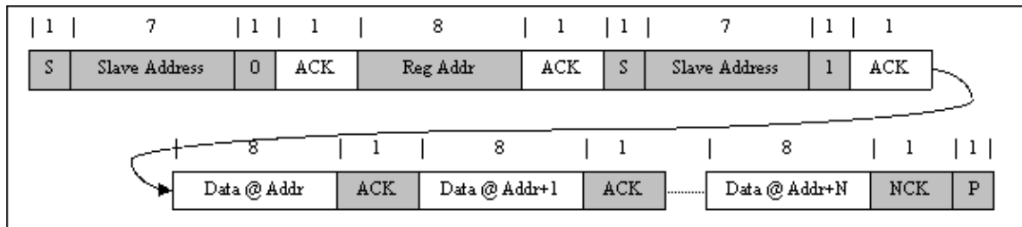
Figure 22. Multi-Read
