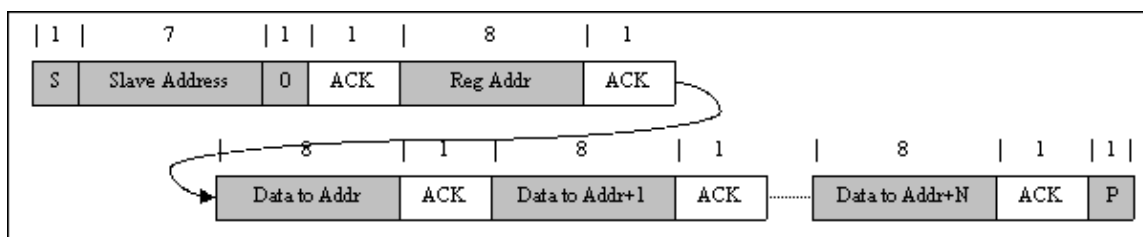
Figure 21. Multi-Write
