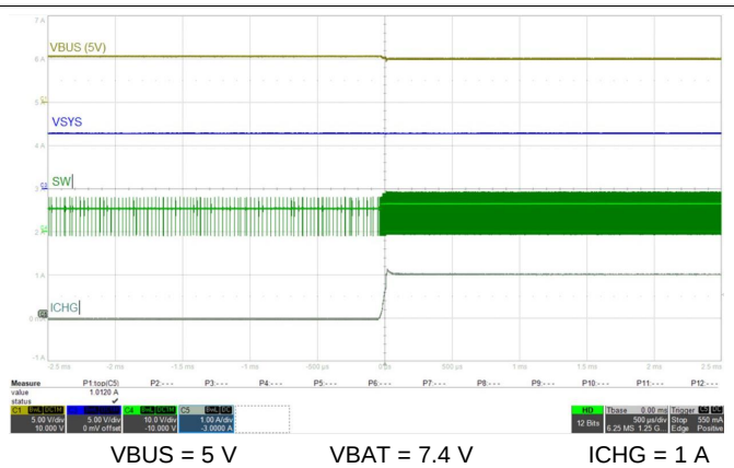
Figure 71. Charge Enable
