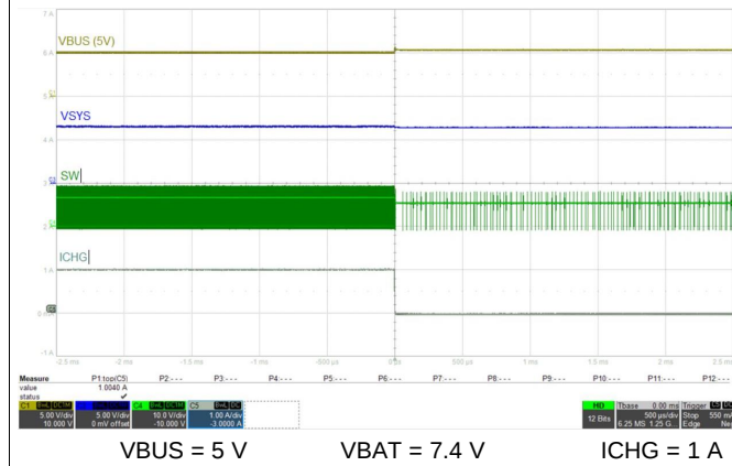
Figure 72. Charge Disabled
