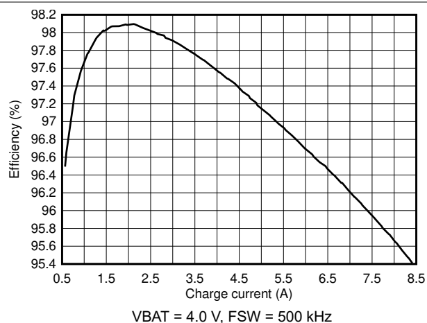
Figure 7-5. Battery Charge Efficiency vs. Charge Current, 3 x 22- \mu F CFLY per Phase
