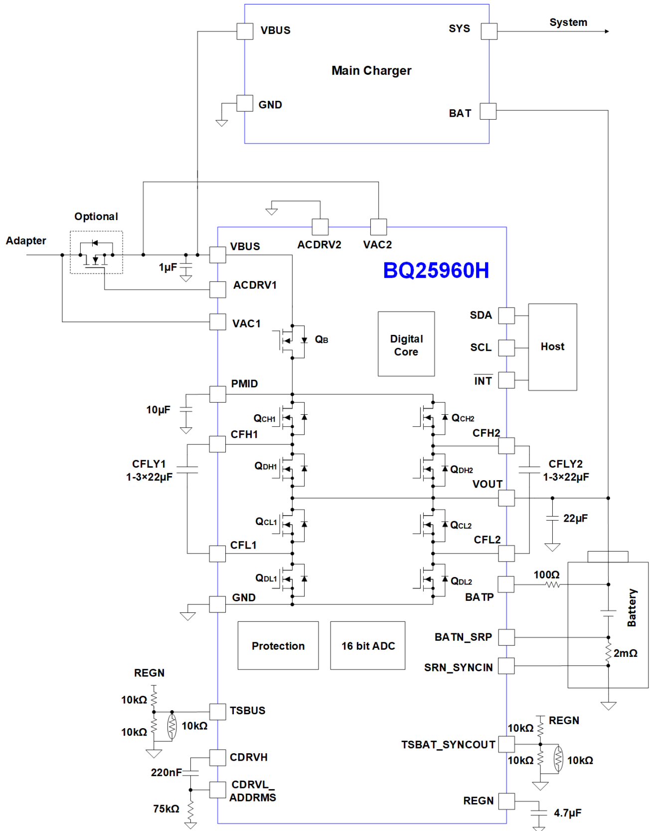
Figure 9-2. BQ25960H Typical Application Diagram with Single Input
