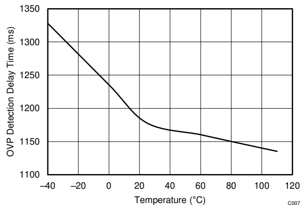
Figure 6-7. OVP Detection Delay Time Versus Temperature
