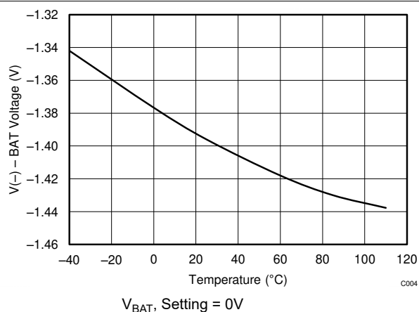
Figure 6-4. 0V Charging Allowed Versus Temperature
