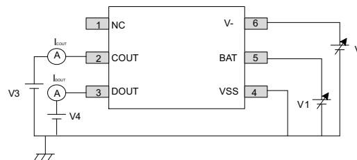
Figure 7-6. Test Circuit 4
