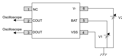
Figure 7-7. Test Circuit 5
