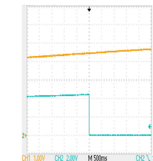
Figure 9-4. Initial Power Up, DOUT
