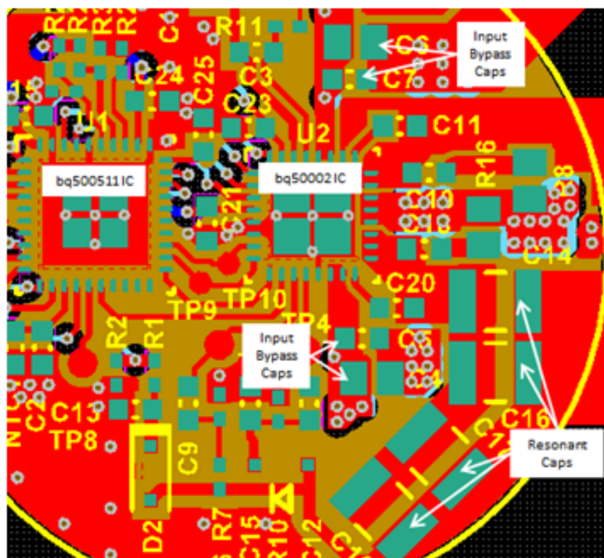
Figure 15. Ground Layout
