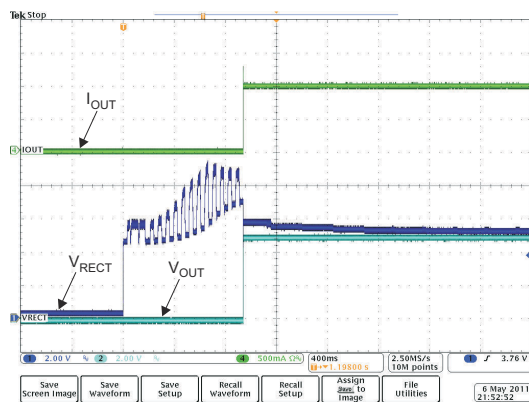
Figure 8-17. BQ51013B-Q1 Typical Start-Up With a 1-A System Load
