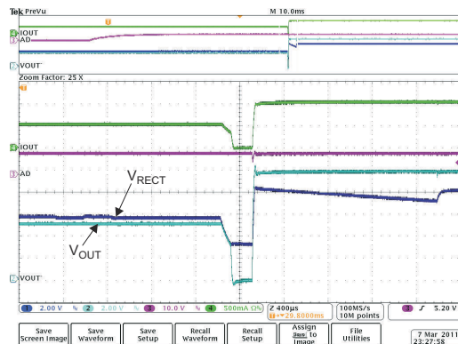
Figure 8-15. Adapter Insertion ( V_{AD} = 10\text{ V} ) Illustrating Break-Before-Make Operation
