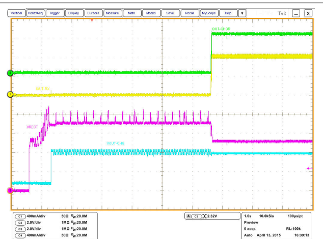
Figure 10-13. System Start-Up With Battery Inserted After Wireless Power is Enabled (1 s / division)
