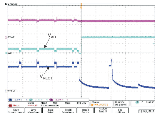
Figure 8-16. On-the-Go Enabled ( V_{OTG} = 3.5\text{ V} ) (3)
