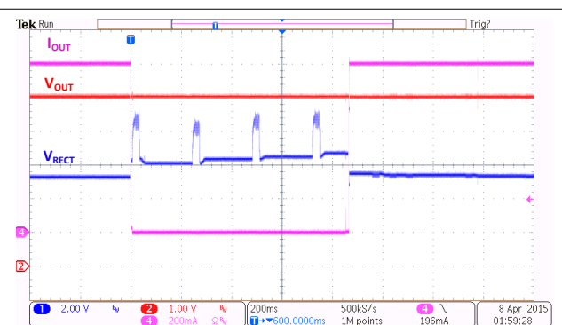
Figure 10-5. Load Transitions (1 A to 0 A to 1 A)
