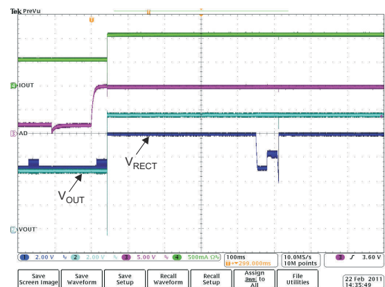
Figure 8-14. Adapter Insertion ( V_{AD} = 10\text{ V} )
