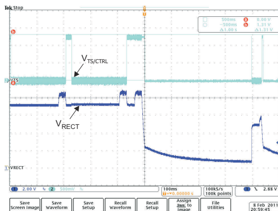
Figure 8-13. TS Fault
