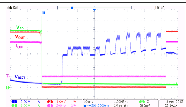
Figure 10-8. Transition Between Wired Power and Wireless Power (EN1 = EN2 = LOW)
