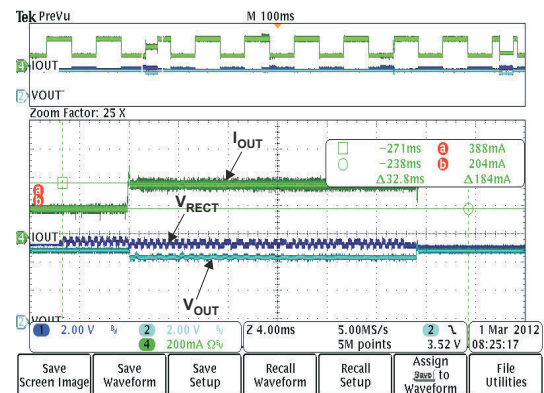
Figure 8-18. Adaptive Communication Limit Event Where the 400-mA Current Limit is Enabled ( I_{OUT-DC} < 300\text{ mA} )
