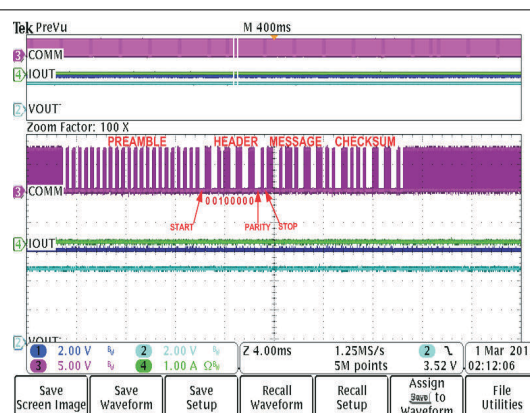
Figure 8-20. RX Communication Packet Structure
