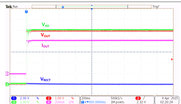
Figure 10-10. AD Power Start-Up With No Transmitter (EN1 = EN2 = LOW)
