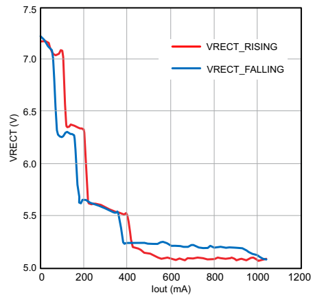
Figure 8-4. Impact of Load Current ( I_{LOAD} ) on Rectifier Voltage ( V_{RECT} )
