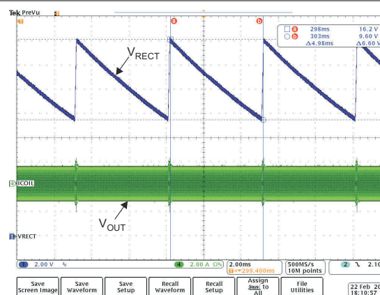
Figure 8-12. Rectifier Overvoltage Clamp ( f_{op} = 110 \text{ kHz} )
