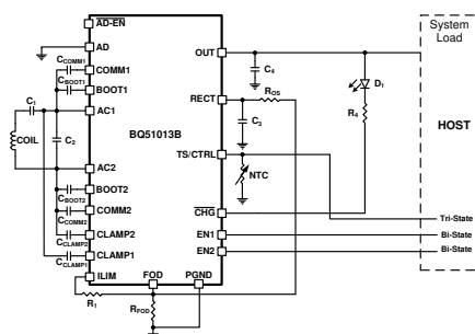
Simplified Schematic
