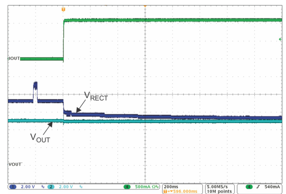
Figure 7-10. 1-A Load Step Full System Response
