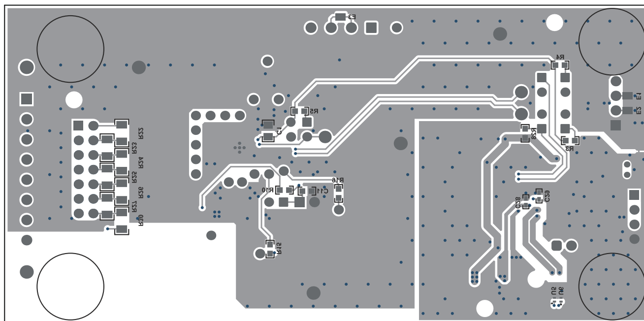
Figure 8-10. BQ76907-Q1 Two-Layer Board Layout—Bottom Layer
