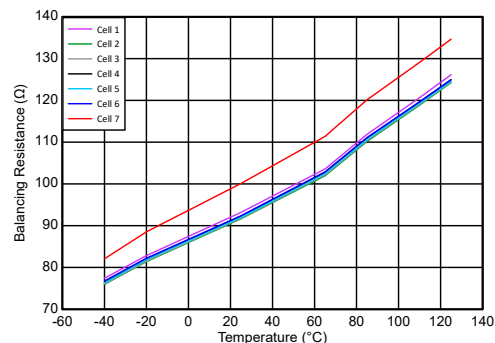
Figure 6-11. Cell Balancing Resistance vs. Temperature
