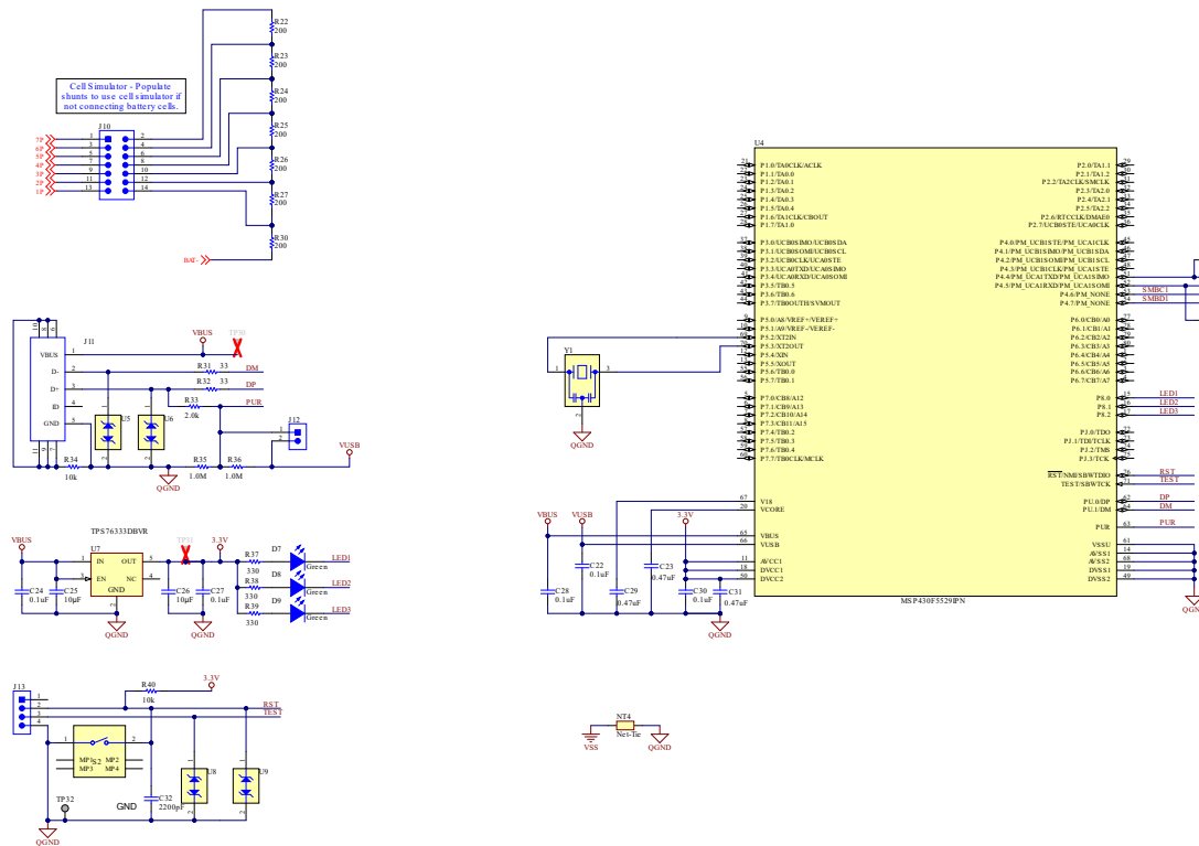
Figure 8-3. BQ76907-Q1 7-Series Cell Schematic Diagram—Additional Circuitry
