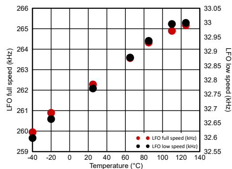
Figure 6-7. Low Frequency Oscillator (LFO) Accuracy vs. Temperature
