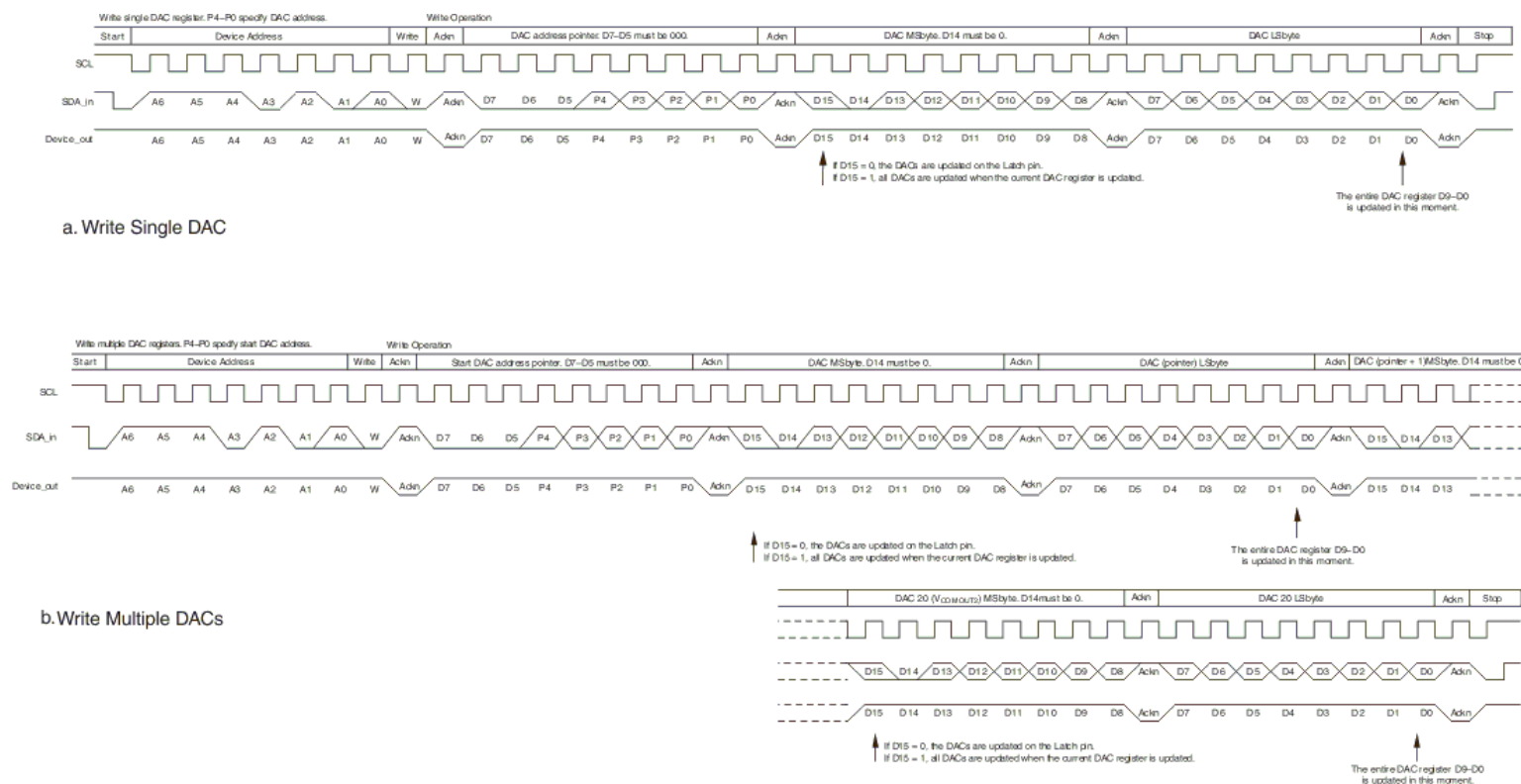
Figure 12. Timing Diagram for Write DAC Register
