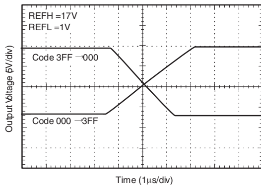
Figure 3. Full-scale Output Swing
