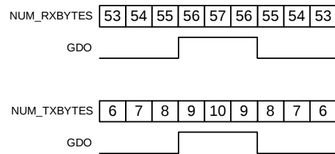
Figure 25: Number of Bytes in FIFO vs. the GDO Signal (GD0x_CFG=0x00 in RX and GD0x_CFG=0x02 in TX, FIFO_THR=13)
