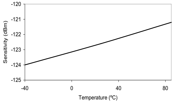
Figure 4-1. Sensitivity vs Temperature
