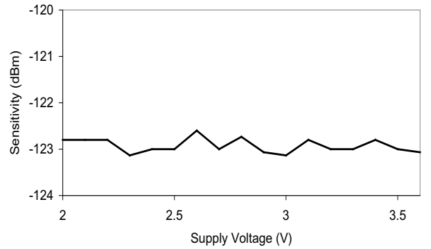
Figure 4-2. Sensitivity vs Voltage
