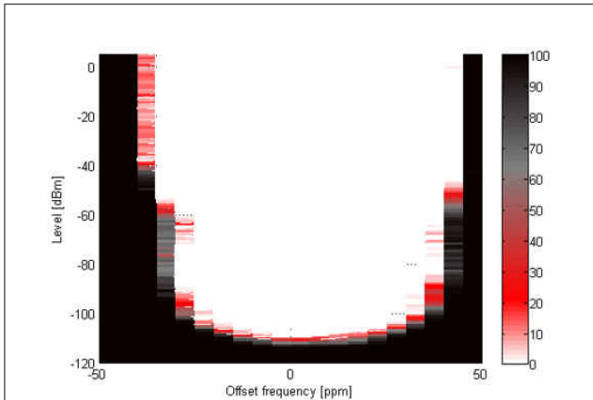
Figure 7-16. PER vs. Level vs. Frequency (SimpleLink™ Long Range 5 kbps, 868 MHz)
