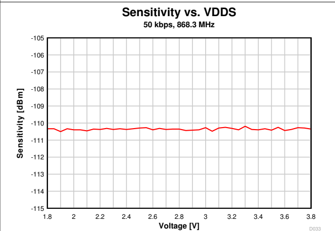
Figure 7-13. Sensitivity vs. Supply Voltage (VDD) (50 kbps, 868.3 MHz)
