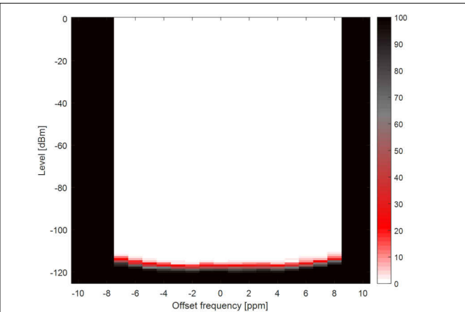
Figure 7-17. Narrowband, 9.6 kbps \pm 2.4 kHz deviation, 2-GFSK, 868 MHz, 17.1 kHz RX Bandwidth
