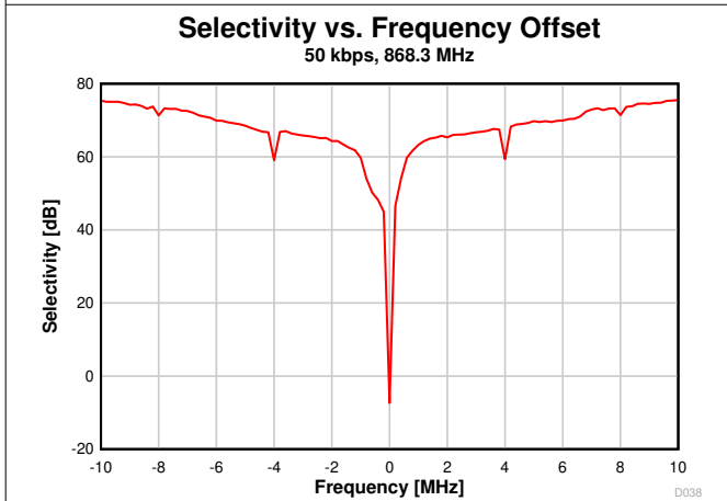
Figure 7-14. Selectivity vs. Frequency Offset (50 kbps, 868.3 MHz)
