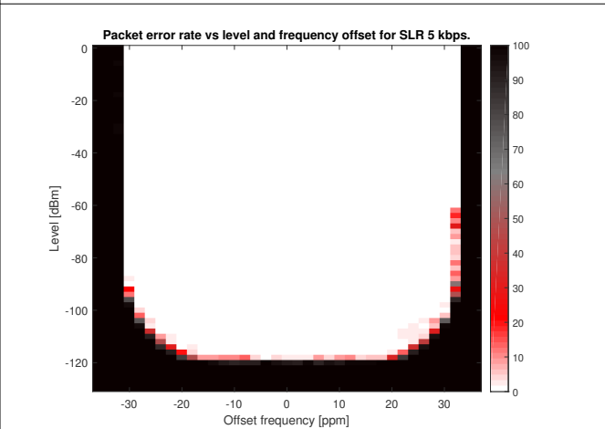
Figure 7-15. PER vs. Level vs. Frequency (SimpleLink™ Long Range 5 kbps, 868 MHz)
