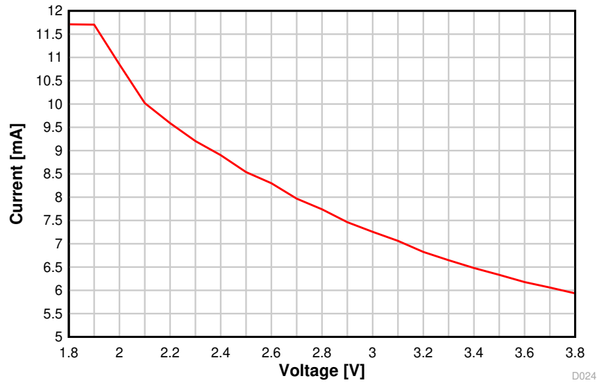
Figure 8-20. TX Current vs. Supply Voltage (VDD5) (BLE 1 Mbps, 2.44 GHz)
