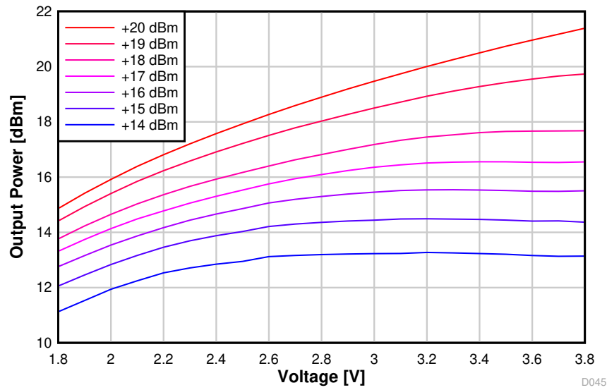
Figure 8-46. Output Power vs. Supply Voltage (VDD5) (50 kbps, 915 MHz)
