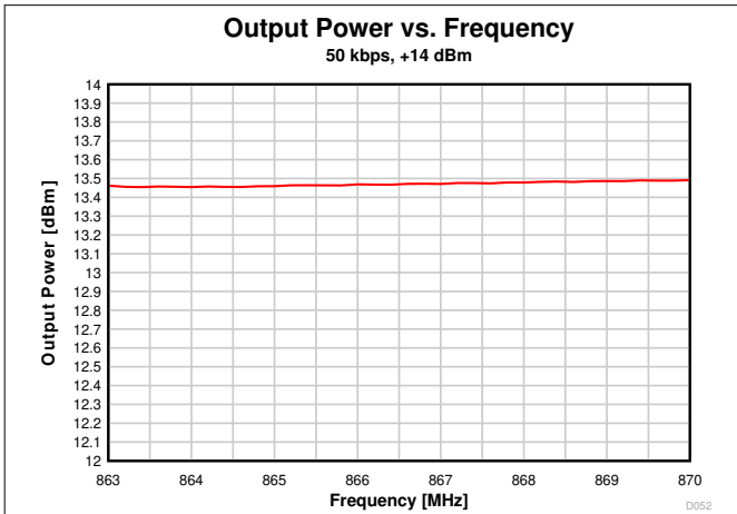
Figure 7-47. Output Power vs. Frequency (50 kbps, 868 MHz)
