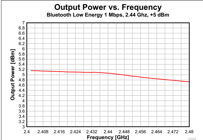
Figure 7-51. Output Power vs. Frequency (Bluetooth Low Energy 1 Mbps, 2.44 GHz, +5 dBm)
