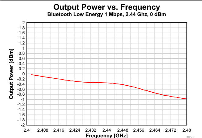
Figure 7-50. Output Power vs. Frequency (Bluetooth Low Energy 1 Mbps, 2.44 GHz)
