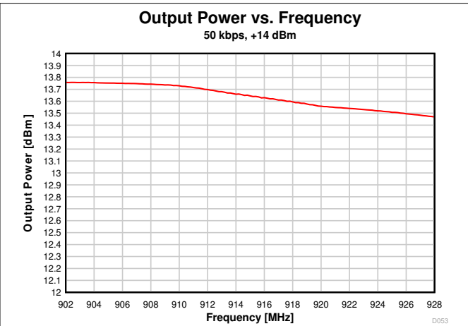
Figure 7-48. Output Power vs. Frequency (50 kbps, 915 MHz)
