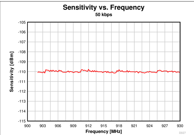
Figure 7-21. Sensitivity vs. Frequency (50 kbps, 915 MHz)
