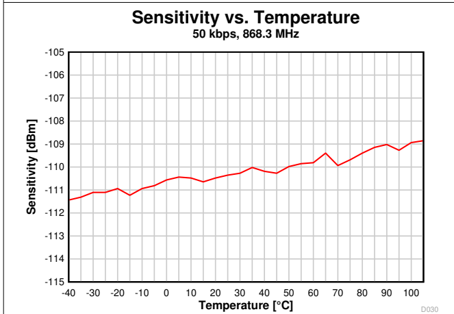
Figure 7-24. Sensitivity vs. Temperature (50 kbps, 868.3 MHz)
