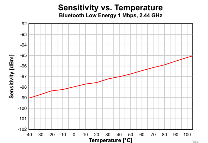
Figure 7-25. Sensitivity vs. Temperature (Bluetooth Low Energy 1 Mbps, 2.44 GHz)
