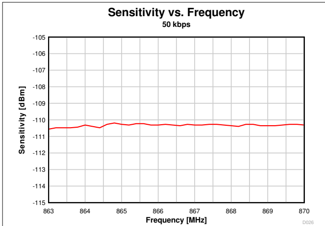
Figure 7-20. Sensitivity vs. Frequency (50 kbps, 868 MHz)
