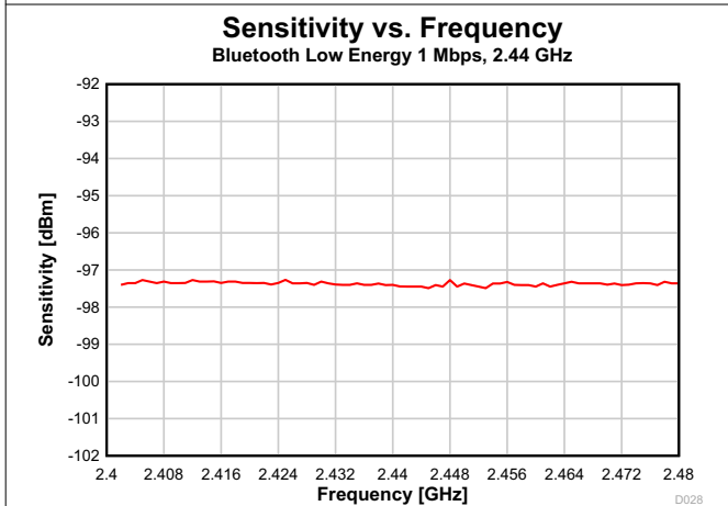
Figure 7-22. Sensitivity vs. Frequency (Bluetooth Low Energy 1 Mbps, 2.44 GHz)
