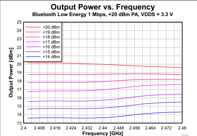
Figure 7-52. Output Power vs. Frequency (Bluetooth Low Energy 1 Mbps, 2.44 GHz, +20 dBm PA)
