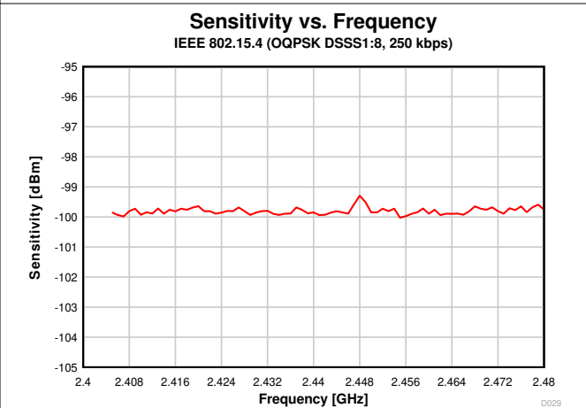
Figure 7-23. Sensitivity vs. Frequency (250 kbps, 2.44 GHz)
