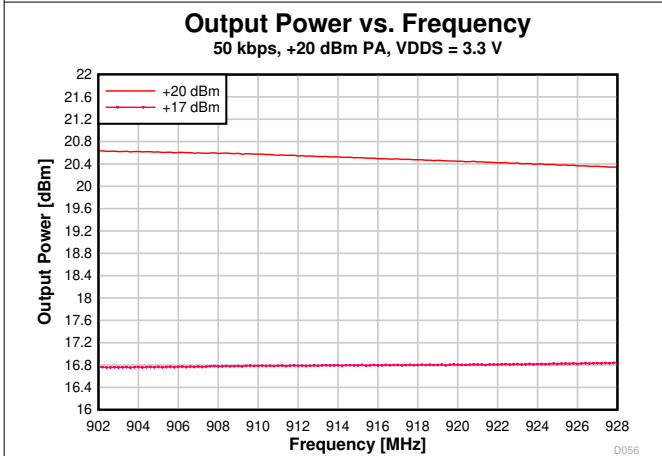
Figure 7-49. Output Power vs. Frequency (50 kbps, 915 MHz, VDD = 3.3 V)
