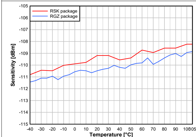
Figure 7-18. Sensitivity vs. Temperature (50kbps, 868.3MHz)
