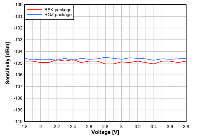
Figure 7-23. Sensitivity vs. Supply Voltage (VDD5) (250kbps, 2.44GHz)
