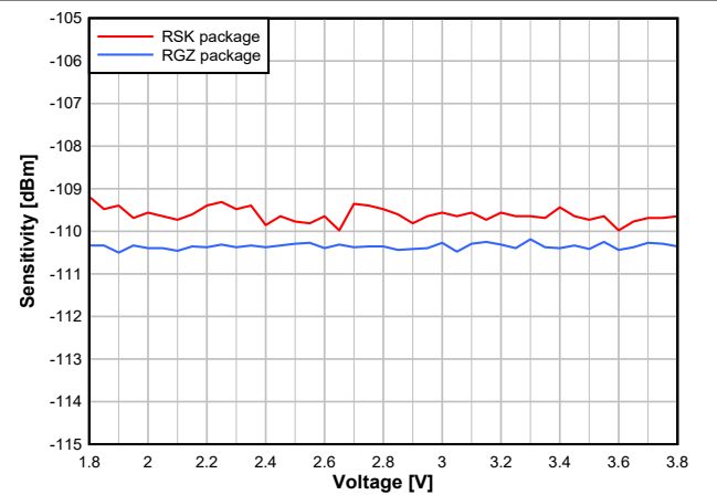
Figure 7-21. Sensitivity vs. Supply Voltage (VDD5) (50kbps, 868.3MHz)
