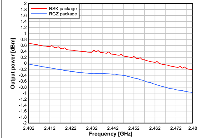
Figure 7-33. Output Power vs. Frequency (BLE 1Mbps, 2.44GHz, 0dBm)
