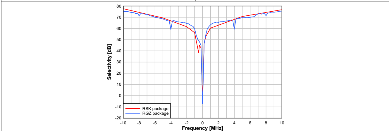
Figure 7-24. Selectivity vs. Frequency Offset (50kbps, 868.3MHz)
