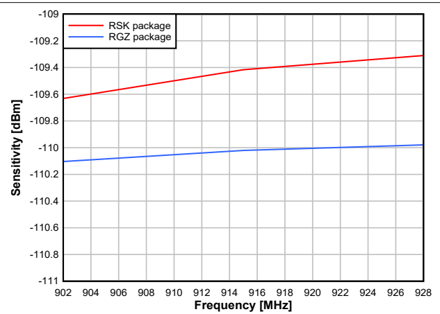
Figure 7-15. Sensitivity vs. Frequency (50kbps, 915MHz)
