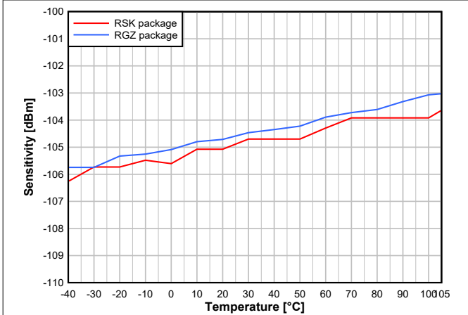
Figure 7-20. Sensitivity vs. Temperature (250kbps, 2.44GHz)
