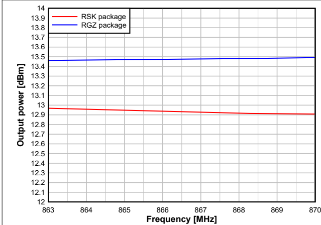
Figure 7-31. Output Power vs. Frequency (50kbps, 868MHz, +14dBm)
