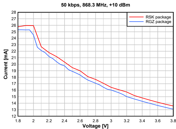
Figure 7-12. TX Current vs. Supply Voltage (VDDS) (50kbps, 868.3MHz)
