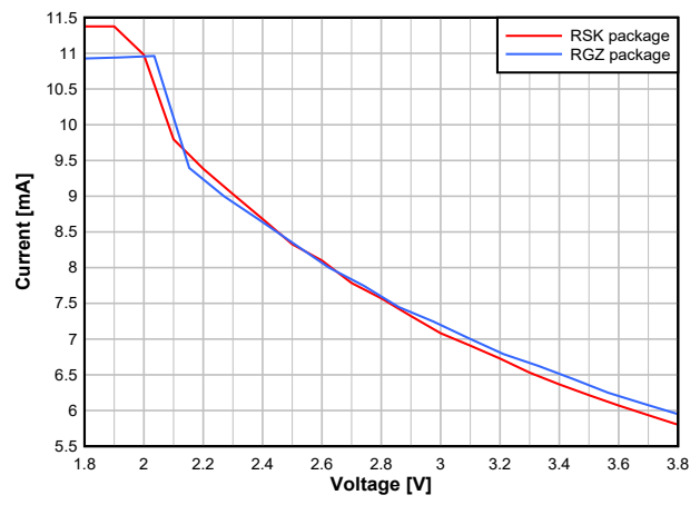
Figure 7-13. TX Current vs. Supply Voltage (VDDS) (BLE 1 Mbps, 2.44GHz, 0dBm)
