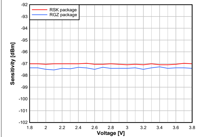
Figure 7-22. Sensitivity vs. Supply Voltage (VDD5) (BLE 1Mbps, 2.44GHz)
