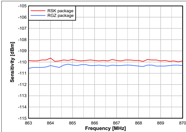
Figure 7-14. Sensitivity vs. Frequency (50kbps, 868MHz)
