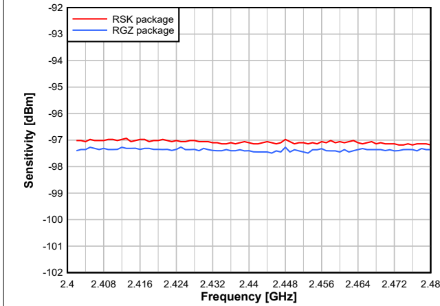
Figure 7-16. Sensitivity vs. Frequency (BLE 1Mbps, 2.44GHz)
