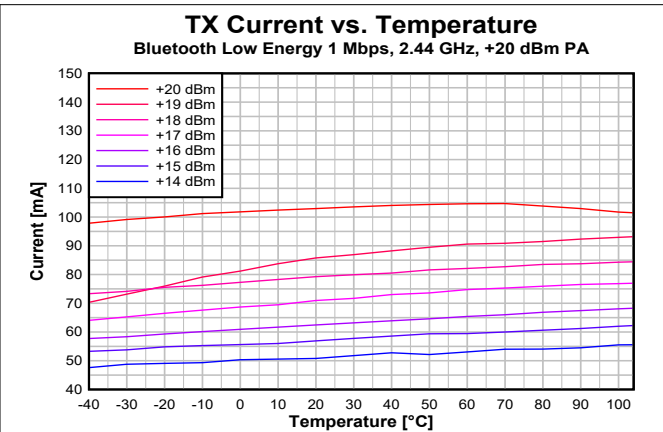
Figure 7-9. TX Current vs. Temperature (Bluetooth Low Energy 1 Mbps, 2.44 GHz, VDD5 = 3.3 V)
