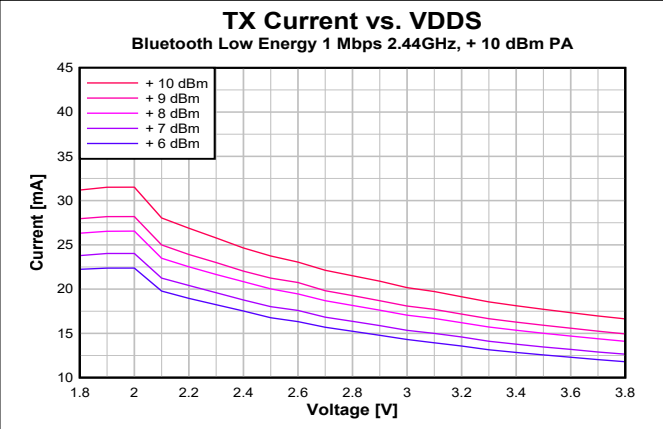
Figure 7-13. TX Current vs. Supply Voltage (VDD5) (250 kbps, 2.44 GHz, +10 dBm PA)
