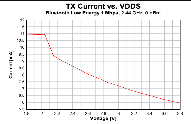
Figure 7-11. TX Current vs. Supply Voltage (VDD5) (Bluetooth Low Energy 1 Mbps, 2.44 GHz)
